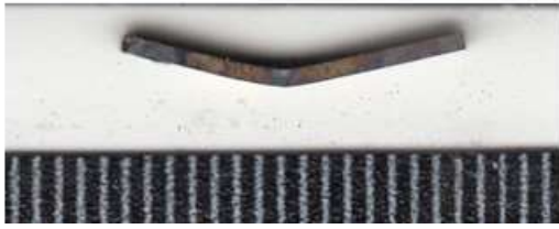
Figure 9. Photograph of the MEA alloy sample after the creep test
