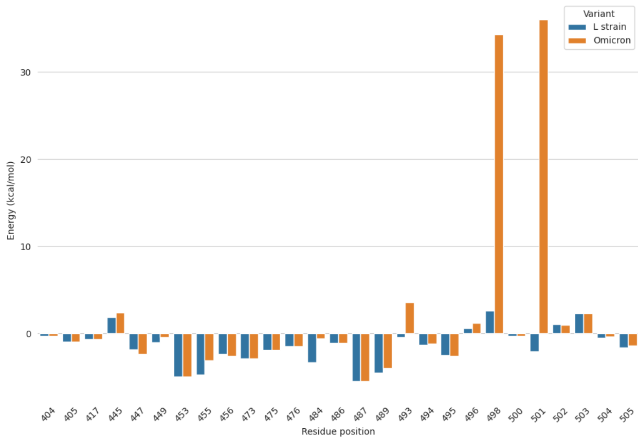
Figure S9. Per residue score breakdown of the L strain and omicron RBD/ACE2 complex form. Scoring was done on the initial backbone of the L strain RBD/ACE2 complex. Mutable interface residues are shown.
