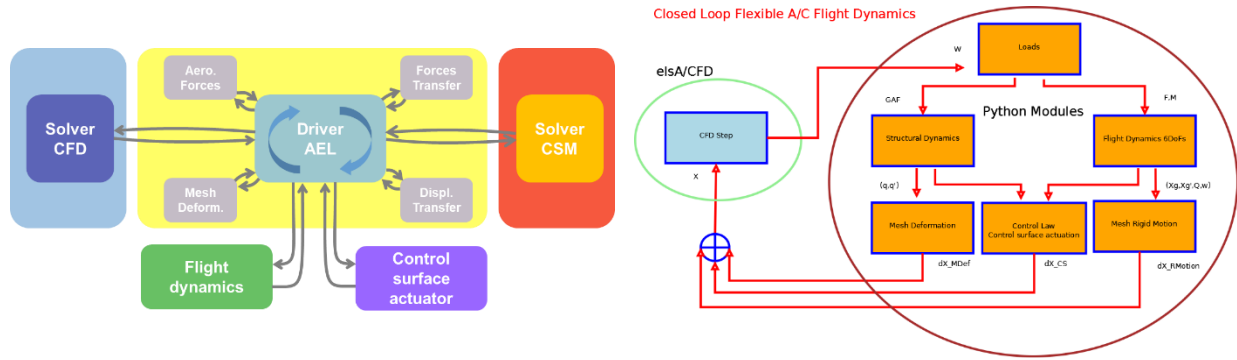
Figure 14: Modular aeroelastic coupling involving additional flight dynamics and surface control actuation modules
