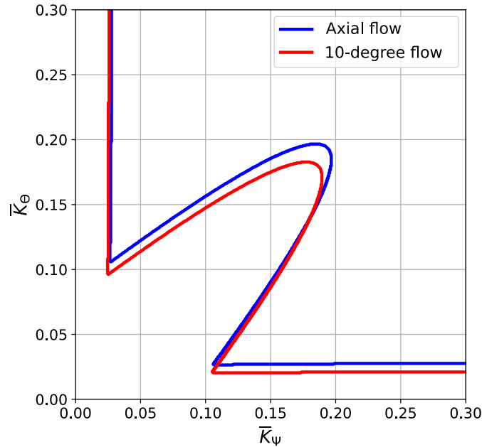
Figure 19: Stability graph with an axial vs non-axial flow (DUST Lifting Line Method simulation).
