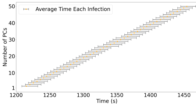
Fig. 2: Average time for each host infected by NotPetya
