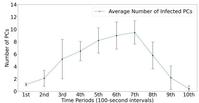
Fig. 4: Number of infected hosts per 100-second period
