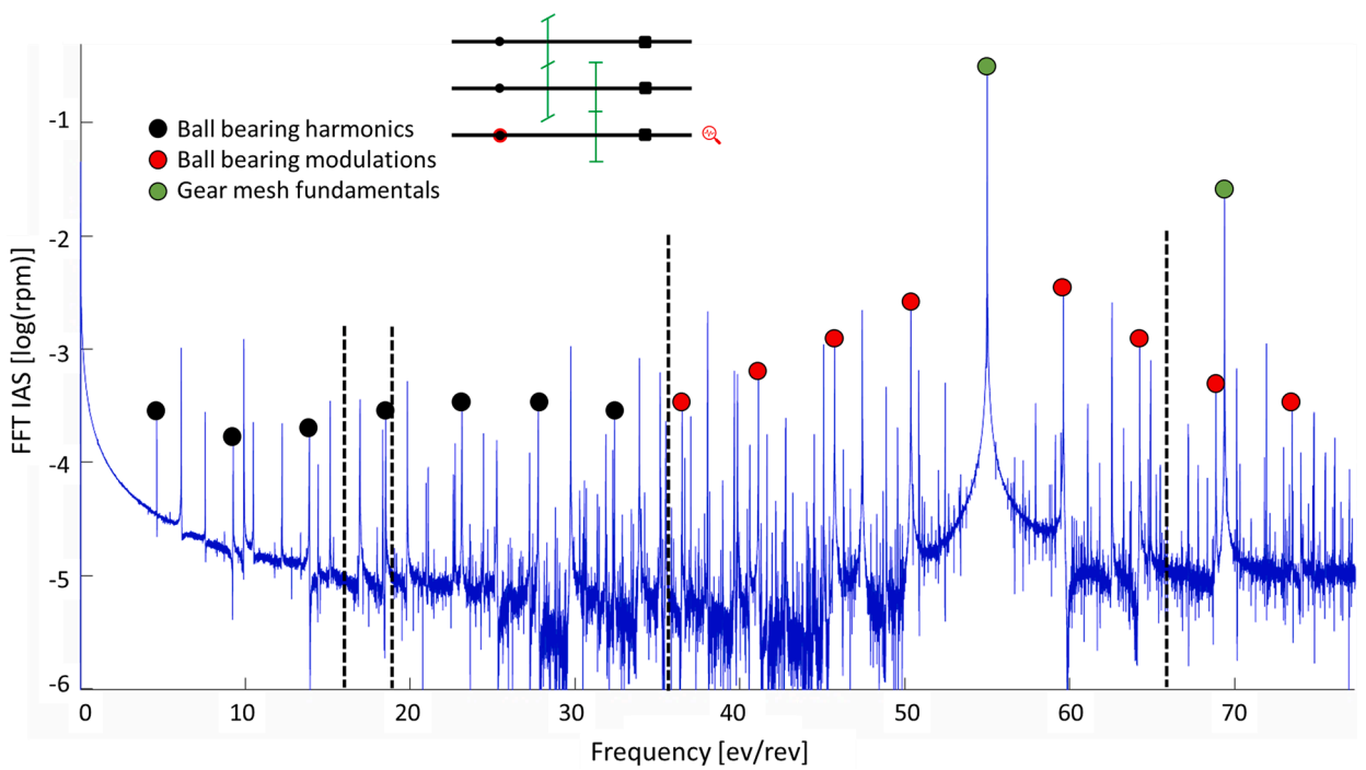
Fig. 11. Angular spectrum of low-speed shaft IAS for a slow and long increase of rotating speed [200 – 900 rpm / 300 rev].
