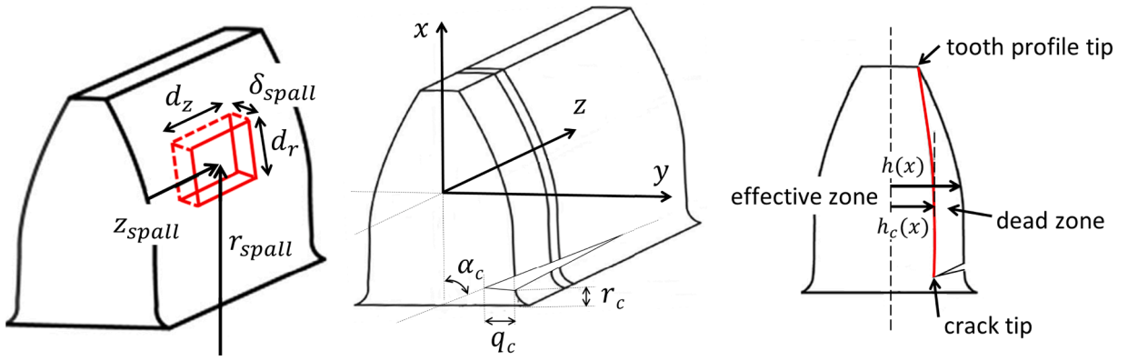
Fig. 5. Implemented damages geometry inspired by [12].
