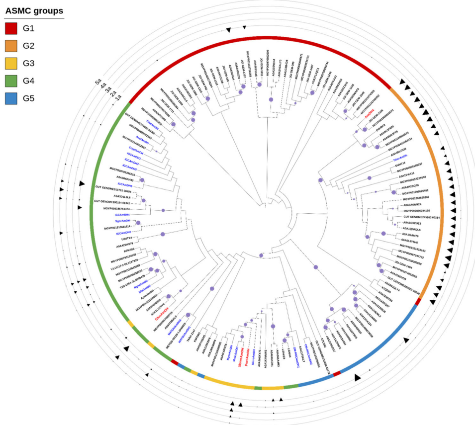
Fig. 4 | Phylogenetic tree of representatives of the extended nat-AmdDH family experimentally tested and their detected activities towards substrates 1a-5a. Tested reference enzymes ( CfusAmdDH , MsmAmdDH , PortiAmdDH and AmdDH4 ) are indicated in red. Active nat-AmdDHs previously reported but not tested in this
