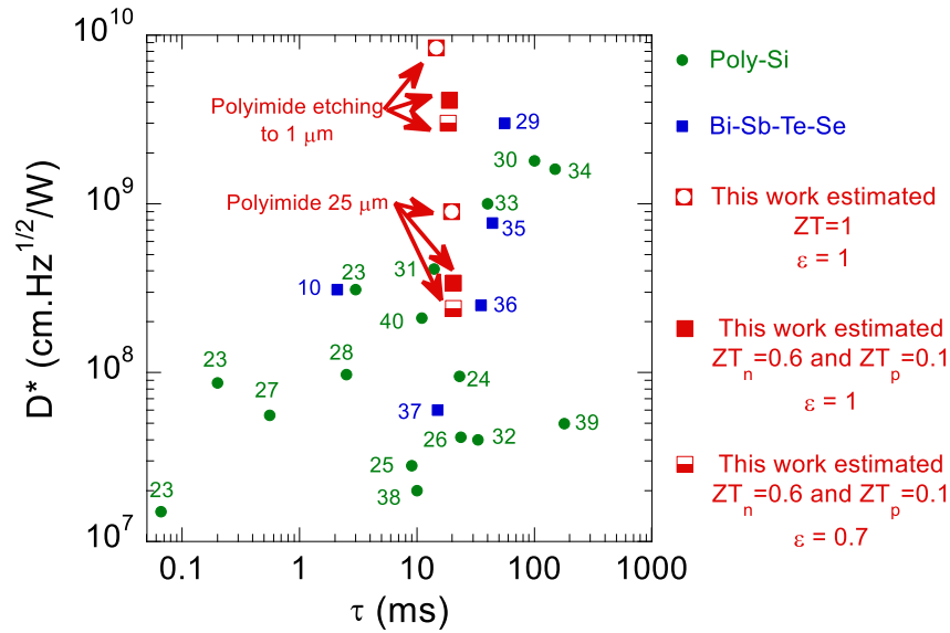
Fig. 4 : Time constants \tau and specific detectivities D^* of TE-bolometers developed with poly-Si [23-28, 30-34, 38-40] (green symbols) and Bi-Sb-Te-Se [10, 29, 35-37] (blue squares) thin films. Estimated specific detectivities on our detector with single junction have been added in the figure (red squares). The estimated values are calculated with ZT_n = 0.6 and ZT_p = 0.1 and for an absorption coefficient of \epsilon \sim 1 (full square), with ZT_n = 0.6 and ZT_p = 0.1 and \epsilon = 0.7 (semi-full square) and with ZT = 1 and of \epsilon = 1 (empty square).
