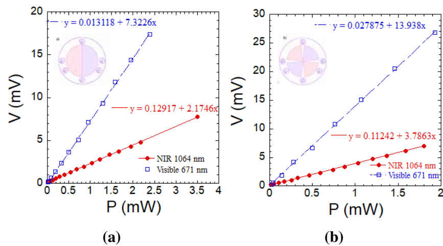
Fig. 2 : Voltage generated versus laser's incident power for visible (blue empty square)) and NIR radiation (red full disk)) for single (a) and dual-junctions (b)
