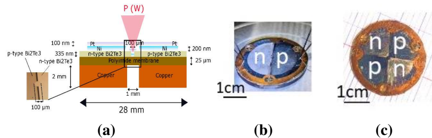
Fig. 1 : Detector characteristics : principle of detector cross section (a) (Scales are not respected) and optical pictures of \text{Bi}_2\text{Te}_3 detectors constituted of single (b) and dual-junctions (c).
