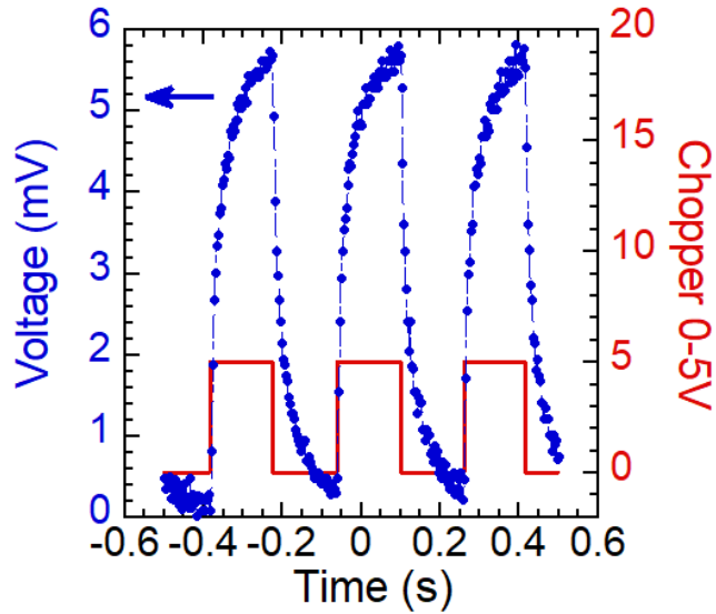
Fig. 3 : Voltage generated for a dual-junctions plotted against time at a frequency of 3 Hz, with NIR radiation of 1.35 mW.
