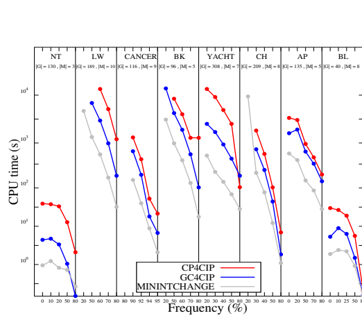
Fig. 1. MinIntChange compared to declarative approaches
