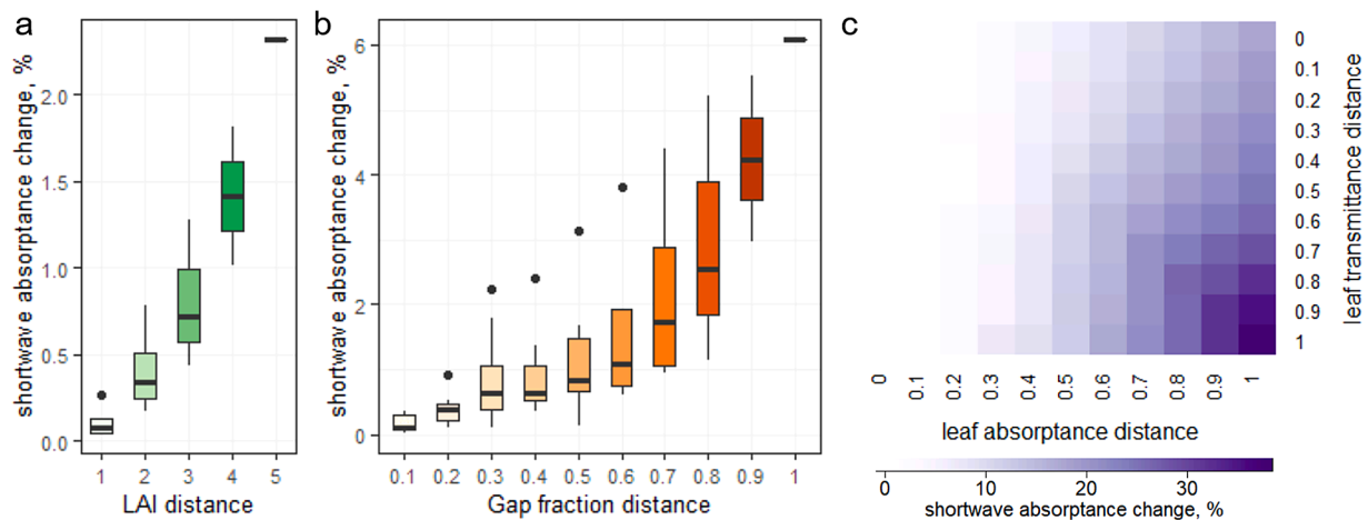
Fig. 5. The change in absorbed radiation in mixtures compared to monocultures as a function of trait diversities (a) for LAI; (b) for LAD represented by the gap fraction distance (the results are presented for natural background, direct sun, and 0^\circ zenith angle parameters); (c) for LOP represented by leaf absorptance and transmittance diversities;
