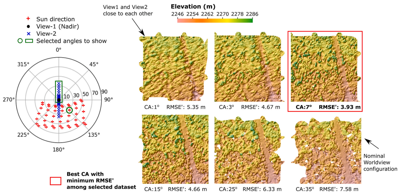
Fig. 6. Influence of convergence angle (CA) on DSM accuracy, measured as RMSE' relative to DSM_{ref} for GPNA. Sample simulations had fixed time (8 AM local 20 June 2013, SZA = 46.42°, SKYL = 33%) and view azimuth angle (180°, from south). The DSM with the lowest RMSE' (3.93 m) had a CA of 7° (red outline). (For interpretation of the references to colour in this figure legend, the reader is referred to the web version of this article.)
