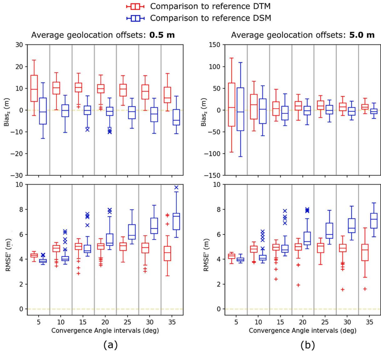
Fig. 9. Influence of axial geolocation offsets with averages of 0.5 m (a) and 5.0 m (b) on the vertical bias and RMSE' of DSMs for the GPNA site for different CAs.
