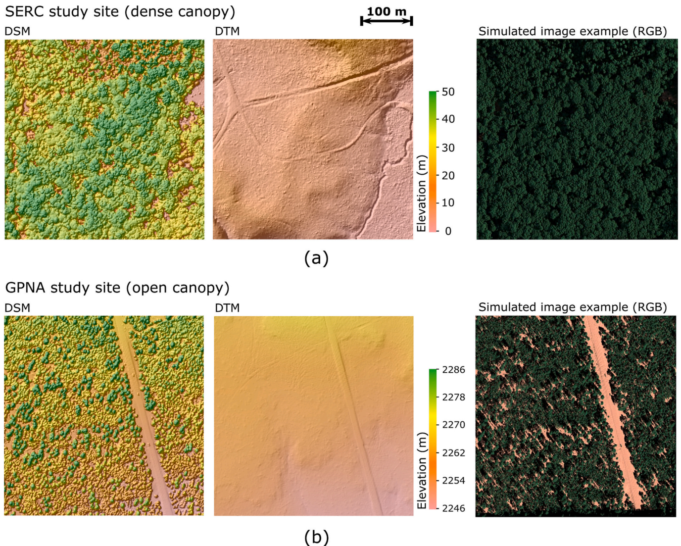
Fig. 1. DSM (left), DTM (center) and DART-simulated image (right, the true colour RGB bands of WorldView) for the study sites (a) Smithsonian Environmental Research Center (SERC), and (b) Gus Pearson Natural Area (GPNA).
