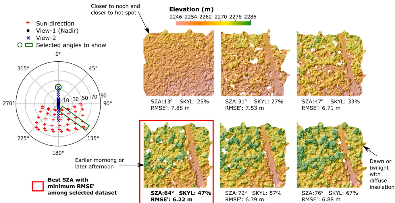
Fig. 5. Sample of generated DSMs with associated RMSE' (to DSM_{ref} ) for stereopairs with different SZA over GPNA. For the selected simulations, the CA is fixed at 35° (viewing from the south), and the selected dates and times capture a small variation range in the solar azimuth angle. The best SZA (64°, SKYL: 47%, 8 AM local on 20 October 2013) among the selected datasets is outlined in red, with an RMSE' = 6.22 m. (For interpretation of the references to colour in this figure legend, the reader is referred to the web version of this article.)
