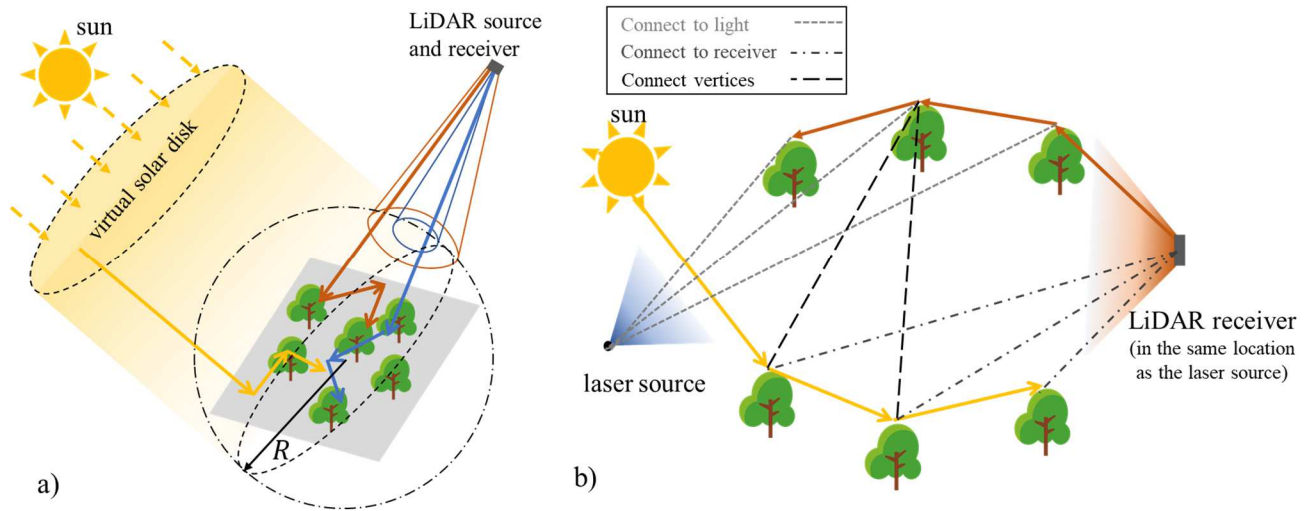
391 a) 392 Fig. 4. Direct light sampling strategy in a “2 sources + 1 receiver” configuration. a) The light sub-path starts 393 from the sunlight (yellow line) or laser source (blue line). The receiver sub-path starts from the LiDAR receiver 394 (orange line). b) One example of direct light sampling: the laser source is selected in “Connect to light” and the 395 sunlight is selected in “Connect to receiver”.
