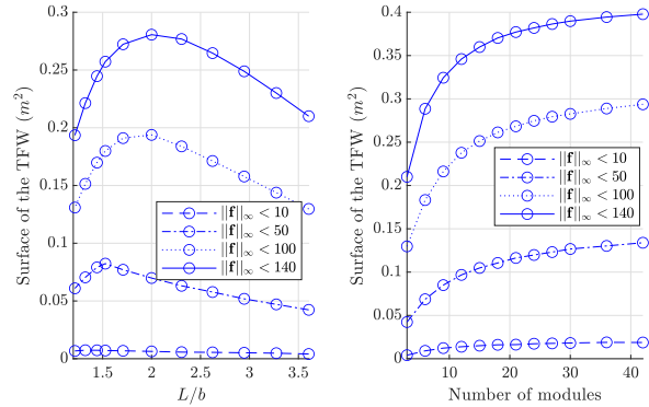
Fig. 8. Evolution of the TFW surface for manipulators with 3 modules as a function of the module ratio L/b (left) and for manipulators without offset as a function of the number of modules (right). Plots are provided for 4 maximum actuation forces.
