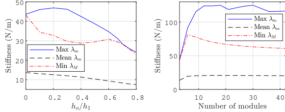
Fig. 10. Evolution of the maximum and mean \lambda_m and the minimum \lambda_M across the TFW for manipulators with 3 modules as a function of the offset height (left) and for manipulators without offset as a function of the number of modules (right).
