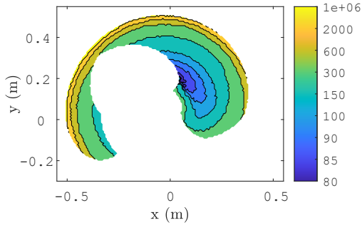
Fig. 6. Distribution of \lambda_M (in N/m) in the TFW in position with minimal forces.
