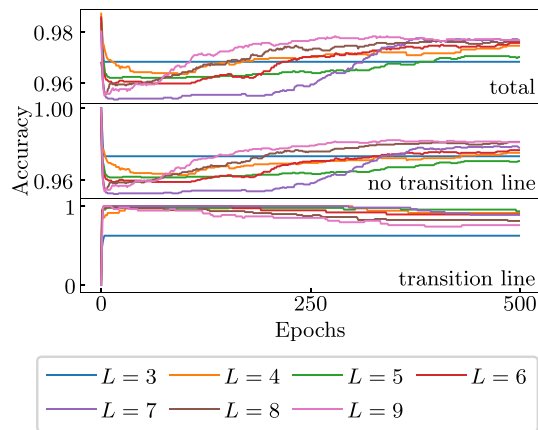
Figure A2. Neural network classification accuracy as a function of training epochs for different input patch sizes. The total accuracy (upper panel) and the accuracies for correctly classifying patches without (centre panel) and with (lower panel) transition lines are plotted as a function of the network training epochs for different sizes of input patches with L \times L pixels (different colours). Convergence is observed for \geq 400 training epochs in all cases.
