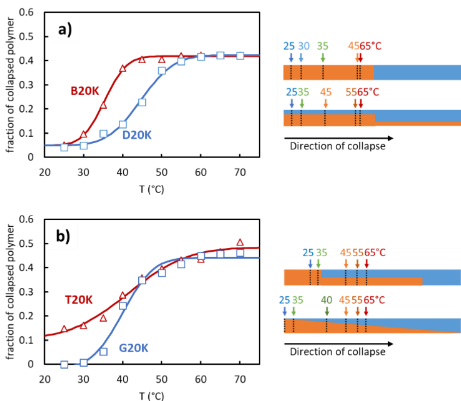
Figure 4. Fraction of collapsed polymer (assuming a progressive chain collapse from the C 12 H 25 terminus) as a function of temperature for the investigated copolymers: a) B20K and D20K; b) T20K and G20K. Open symbols represent experimental points derived from NMR measurements, while the solid curves represent the best fit of a 4-parameter sigmoidal function used to establish the location and breadth of the thermal transition. On the right side of both plots, there is a schematic representation of the fraction of collapsed polymer at different temperatures.
