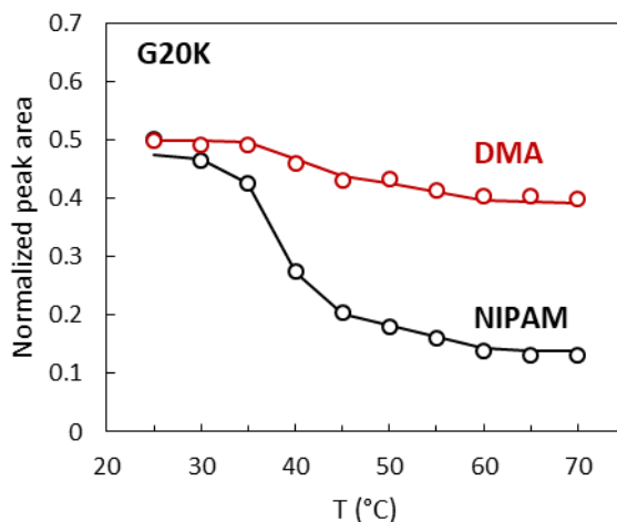
Figure 3. Progressive polymer chain collapse in aqueous solution as a function of temperature for copolymer G20K. Red and black circles show the normalized integral value of the ^1\text{H} NMR signals for DMA and NIPAM, respectively. Red and black lines show the predicted normalized integral value of the ^1\text{H} -NMR signals for the corresponding fraction of collapsed polymer based on the copolymer composition profile (see section S3 in SI for details).
