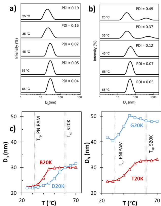
Figure 2. Intensity weighted size distributions of hydrodynamic diameters measured by DLS at different temperatures for B20K (a) and G20K (b); c) Z-average hydrodynamic diameters as a function of temperature for all copolymers. Dashed lines at 32 °C and 60 °C correspond to the cloud point temperature of PNIPAM and 1:1 P(NIPAM-co-DMA) statistical copolymer, respectively.
