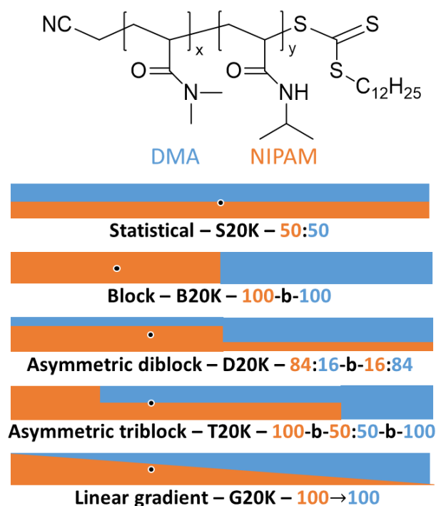
Figure 1. Schematic representations of the chemical formula and of the investigated NIPAM-DMA copolymer composition profile. The orange fraction represents the proportion of NIPAM in the copolymer along the chain: for example, it is constant in the statistical copolymer in which NIPAM is randomly mixed with DMA; it varies gradually from one end, mainly composed of NIPAM, to the other, mainly composed of DMA, in the case of linear gradient copolymer; The center of mass of the distribution of NIPAM monomer units within the copolymer is represented by a black dot (see SI for more details).
