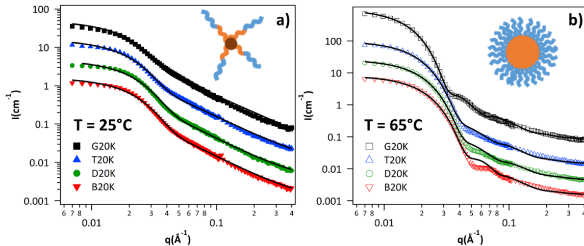
Figure 5. Neutron scattering intensity as a function of the scattering vector for the different copolymers with molar mass of 20kDa at a) T = 25\text{ }^{\circ}\text{C} and b) T = 65\text{ }^{\circ}\text{C} ; the curves have been arbitrarily shifted to facilitate comparisons. The black solid lines are the fitted curves using the Dozier model at T=25^{\circ}\text{C} and core-shell model (homogeneous core and decaying density profile in the shell) at T=65^{\circ}\text{C} .
