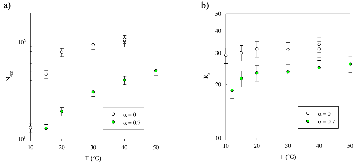
Figure 3. Evolution of a) the aggregation number and b) the hydrodynamic radius of Ran as a function of temperature for C = 5 g/L, [Na + ] = 0.1 M and \alpha = 0 (O) or \alpha = 0.7 (●).
