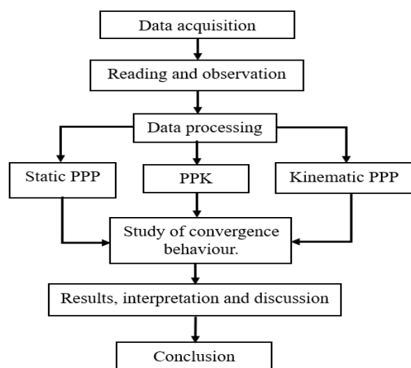
Figure 1. Methodology chart
