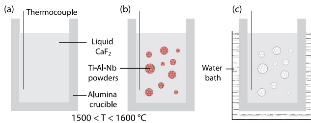
Fig. 3. Experimental schematic for heat treatment of particles, (a) molten salt at temperature, (b) addition of particles and (c) quenching.
