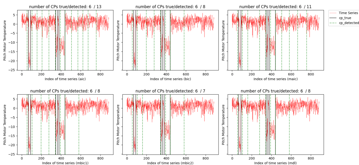
Figure 9. Pitch motor temperature signals with six labeled change points (in vertical solid black lines).
