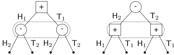
Figure 2: Two EFGs for Matching Pennies.
