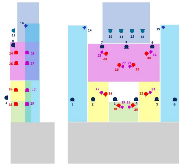
Fig. 6: Microphone installation (left) side and (right) frontal views, Saint-Sulpice organ case.
