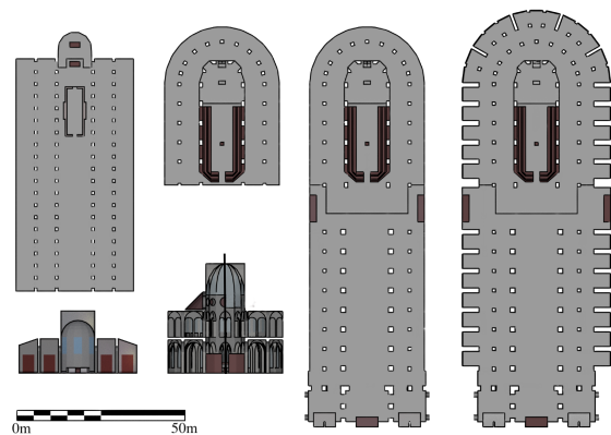
Fig. 1: Acoustic model floor-plans and sections of cathedrals built on Île-de-la-Cité, from left to right: the pre-Gothic basilica underneath Notre-Dame's parvis (before 1163); Notre-Dame at its consecration (1182); completion of the nave (ca. 1220) and lateral chapels (ca. 1350).
