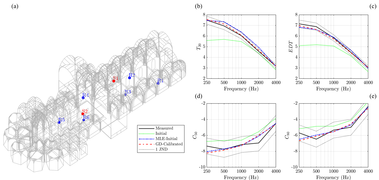
Fig. 1: (a) GA model of Saint-Germain-des-Prés with the source-receiver locations used in the calibration. Averaged values of room metrics including (b) T_{20} , (c) EDT, (d) C_{50} , and (e) C_{80} , during the calibration procedure.
