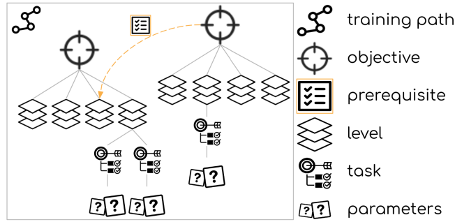
Fig. 1: Knowledge Structure [18]
