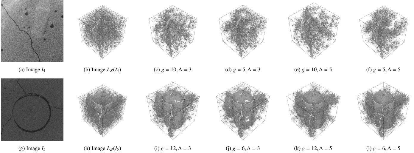
Figure 7: The input images I_4, I_5 and the crack detection results produced by our method.
