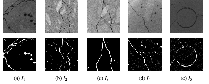
Figure 2: First row: Slices of input gray scale images I_j, j = 1, \dots, 5 . Second row: Corresponding slices of binary images L_S(I_j), j = 1, \dots, 5 computed using the Maximal Hessian Entry filter.
