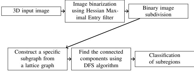
Figure 1: 6-step process diagram for crack localization in 3D concrete images
