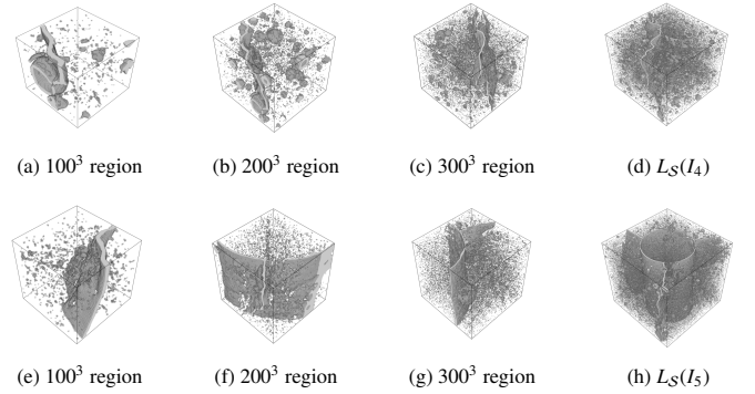
Figure 3: 3D visualization of subregions \tilde{W} of different size of binary images L_S(I_4) and L_S(I_5) .
