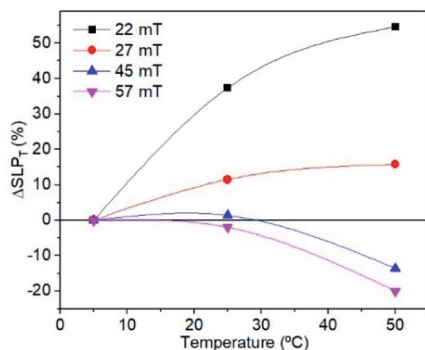
Fig. 9 Evolution of the \Delta\text{SLP}_T of sample MAG-30 as a function of T_i for different fields and t = 10 s.
