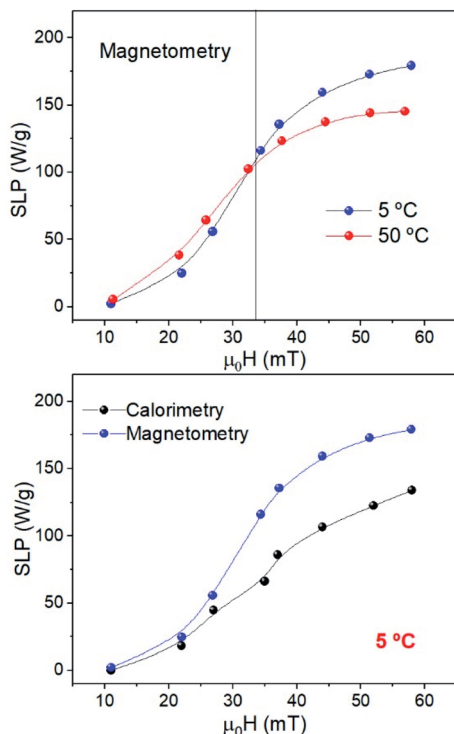
Fig. 11 (Above) SLP vs. the field of sample MAG-30 obtained by AC-magnetometry at T_i = 5\text{ °C} and 50\text{ °C} (the black line is only to guide the eyes) and (below) comparison between calorimetry and AC-magnetometry for sample MAG-30 at T_i = 5\text{ °C} .
