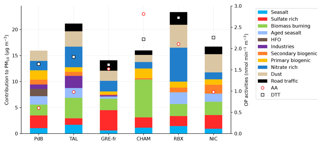
Figure 3. The contribution of sources to PM_{10} and the OP activities in six sites. The left y axis and bar show the contribution of PM sources in \mu\text{g m}^{-3} . The right y axis, circles, and squares show the mean OP_V activities in \text{nmol min}^{-1} \text{m}^{-3} , with the red circle indicating OP_{AA} and the black square indicating OP_{DTT} .
