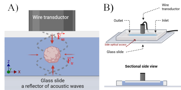
Fig. 1. Sketch of the acoustofluidic chip (A) Side view of the acoustofluidic chip showing the standing acoustic wave inside the PDMS cavity. The typical frequency is 2\text{ MHz} , corresponding to an acoustic wavelength \lambda_{ac} \approx 375\ \mu\text{m} . The axial force F_{ax} is 10 times stronger than the transverse force F_{tr} . The acoustic wave propagates in water and the reflector is a 1\text{ mm} thick glass slide. (B) Top view and side view of the PDMS chip with the acoustic transducer on top.
