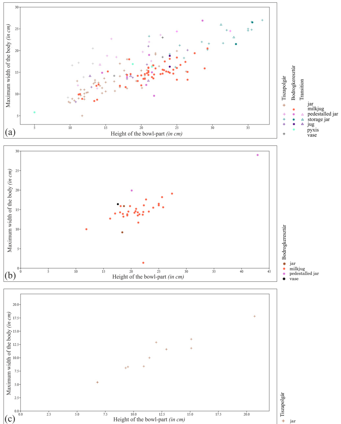
Figure 6: Scatter plot of vessels with neck at: (a) Tiszapolgár-Basatanya; (b) Tiszavalk-Kenderföld; and (c) Polgár-Nagy-Kasziba and Tiszabólna-Szilpuszta (the legends contain the traditional typological terms to visualise their metrical distribution).
