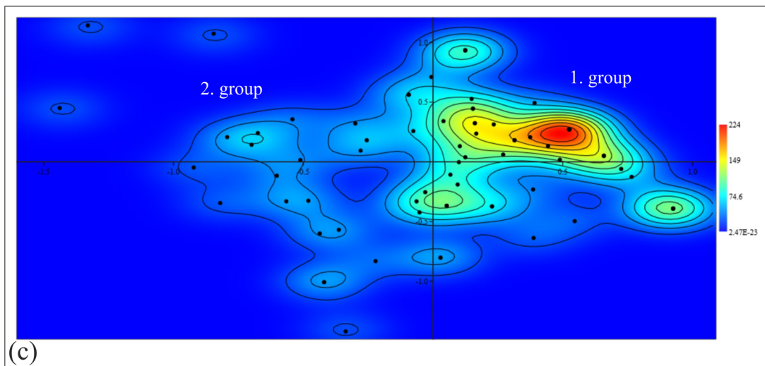
Figure 9: (a) Correspondence analysis of the graves from Tiszapolgár-Basatanya with 1\sigma ellipse and the separation of the transitional graves. (b) Correspondence analysis of the graves from Tiszapolgár-Basatanya with the omission of transitional graves. (c) Kernel density plot generated from the second correspondence analysis from Tiszapolgár-Basatanya.
