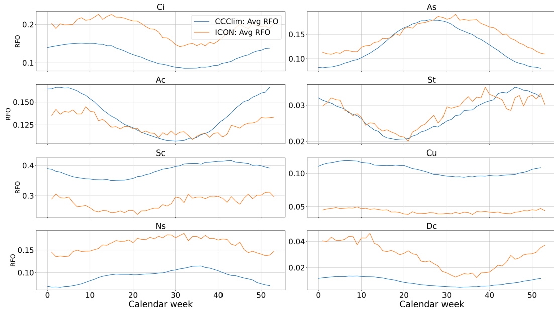
Figure 5. Example comparison of the mean cloud-type RFOs by calendar week over the southern hemispheric oceans between CCCLim (blue) averaged over the full 35-year period and an ICON-A simulation (orange; see Sect. 4) averaged over 2 years.
