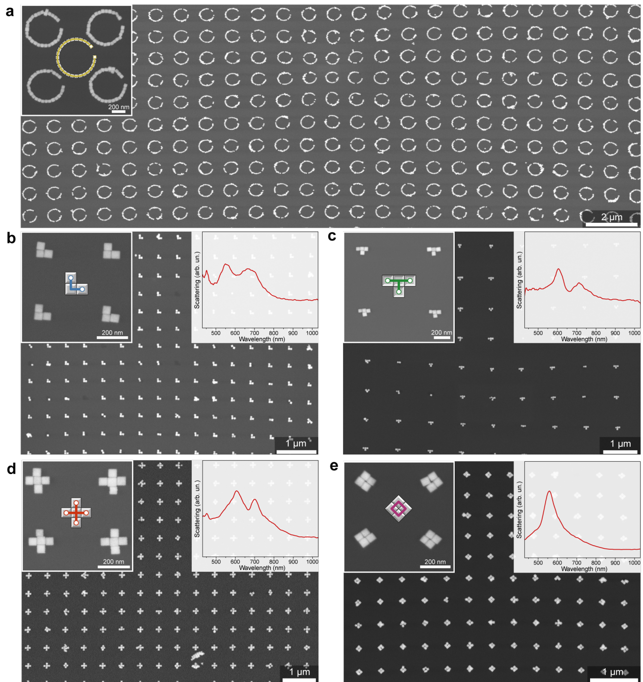
Figure 2: Assembly of 55 nm AgNCs on different basic meta-atoms with their corresponding measured dark-field scattering. a, Split-ring resonator. b, L-shape. c, T-shape. d, Cross-shape. e, Diamond-shape.
