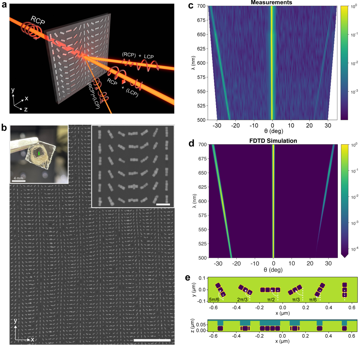
Figure 5: Bottom-up Pancharatnam-Berry metasurface from nanocubes. a, Illustration of wavelength-dependent light steering after RCP light passes through the metasurface. b, Photographic and SEM images of nanocubes assembly on nanopatterned PDMS after the excess nanocubes removal. Scale bars are 200 nm in the inset and 2 \mu\text{m} in the main image. c, Experimental results of steering angle on the wavelength of incident RCP light. d, FDTD simulation results of steering angle on the wavelength of incident RCP light. The intensities for c and d are normalized relative to the peak intensity at each wavelength and are presented on a logarithmic scale (base 10). e, Geometry of simulated meta-atoms in a unit cell.
