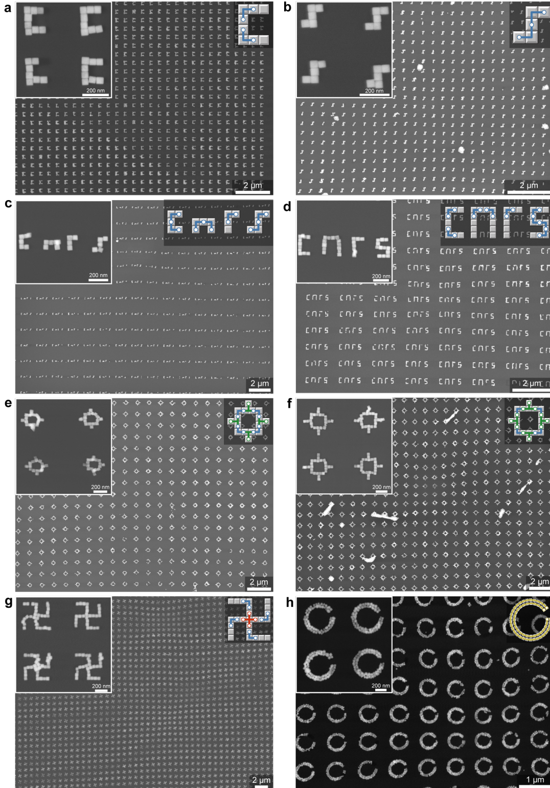
Figure 3: Assembly of 55 nm AgNCs on nanopatterns of a, C-shape, b, S-shape, c-d composed meta-atoms representing the CNRS letters (small and large respectively), e, small polygonal shape, f, larger polygonal shape, and g, chiral gammadion. h, Assembly of 40 nm AgNCs on 80 nm width split-ring pattern.
