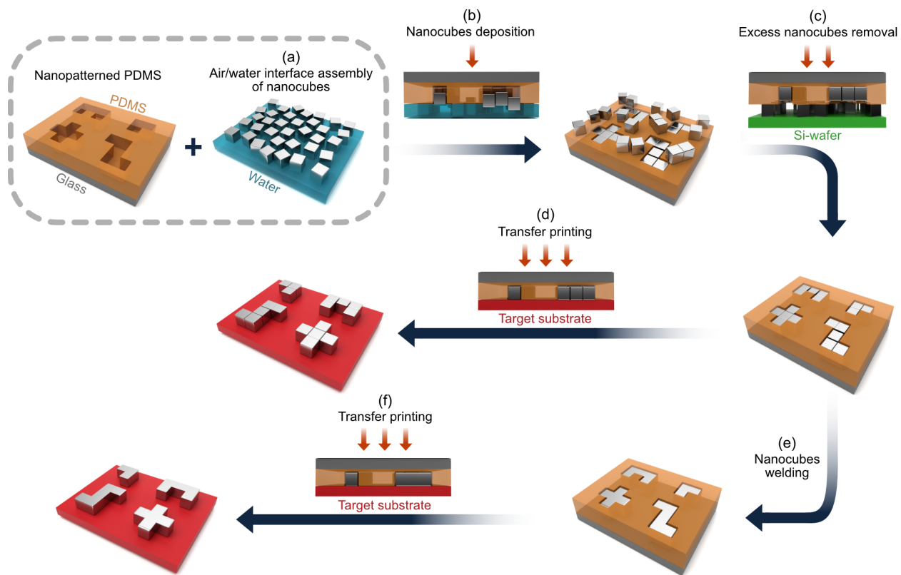
Figure 1: Diagram of nanopattern fabrication from nanocubes. The process involves: a, nanocubes dispersion at the air/water interface, b, nanocubes directed assembly, c, excess nanocubes removal. Subsequent pathways include: d, transfer printing of assembled nanocubes onto target substrate.
