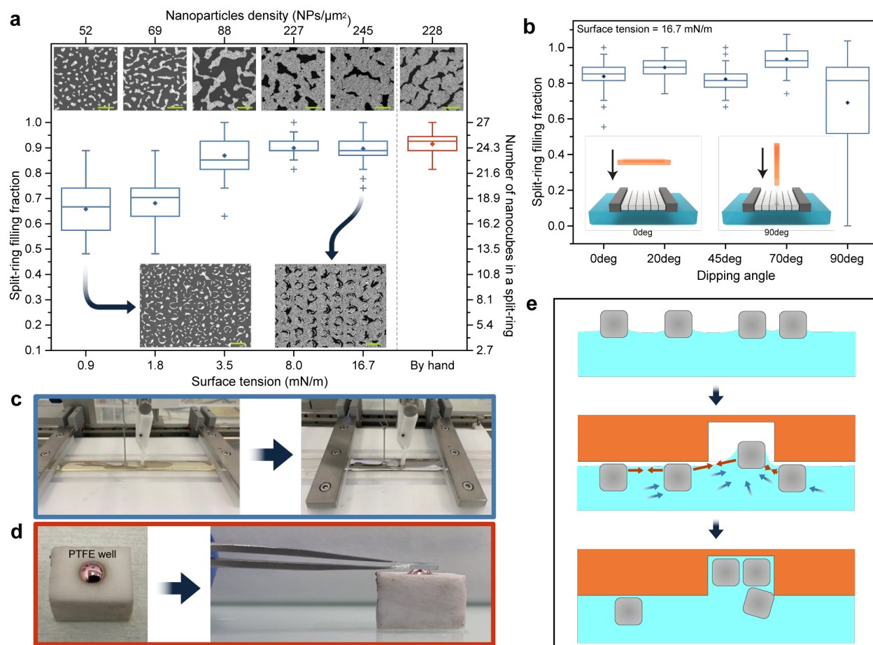
Figure 4: Nanocubes assembly using air/water interface assembly technique. a, Filling fractions of nanocubes inside split-ring nanopattern at different surface tension deposited using a Langmuir trough at 0^\circ dipping angle (blue) vs. using PTFE well by hand (red). The color code of the box plot is the same as that used for c and d. Top insets depict nanocubes density in relation to surface tension on a flat PDMS surface, while bottom insets show density with respect to nanopatterned PDMS surfaces. Scale bars are 1 \mu\text{m} in length. b, Nanocubes assembly at different dipping angles at 16.7 \text{ mN/m} . Insets depict the orientations of nanopatterned PDMS substrate (orange) during nanocubes deposition: horizontal alignment at 0 degree and vertical alignment at 90 degree. Center line: Median. Diamond: Average. Box: Interquartile range. Whiskers: Maximum and minimum. Crosses: Outliers. N = 42\text{-}63 samples. c, Nanocubes assembly using Langmuir trough with automated deposition. d, Nanocubes assembly using PTFE well with manual deposition by hand. e, Proposed mechanism of nanocubes filling. Light blue color indicates water subphase, orange color indicates nanopatterned PDMS substrate, dark blue arrows indicate water flux, and red arrows indicate attractive capillary forces.
