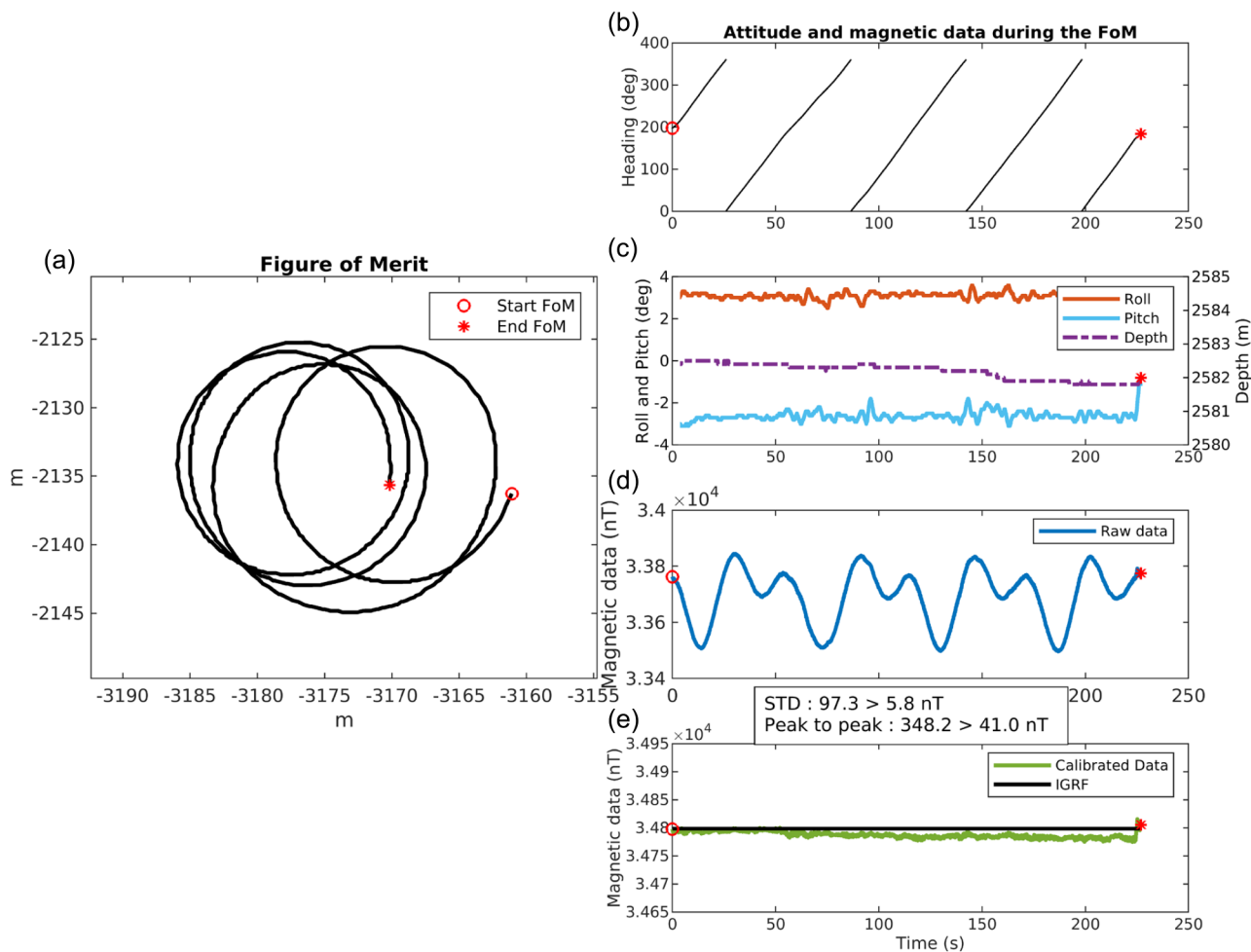
FIGURE 10 Path of a figure of merit of Sentry autonomous underwater vehicle (AUV) (a). Time series of drone heading (b) and depth, pitch and roll (c), and raw (d) and calibrated (e) magnetic data. Intensities of the magnetic data are given in nT, heading, roll and pitch angles in degrees and depth in metres. The standard deviation between the norms of the raw total magnetic intensity (TMI) and the International Geomagnetic Reference Field (IGRF) is 97.3 nT and is reduced to only 5.8 nT for the calibrated data. Peak-to-peak ranges similarly decrease from 348.2 nT before calibration to 41.0 nT after. STD, standard deviation of differences. Source: IGRF data are from Alken et al. (2021).
