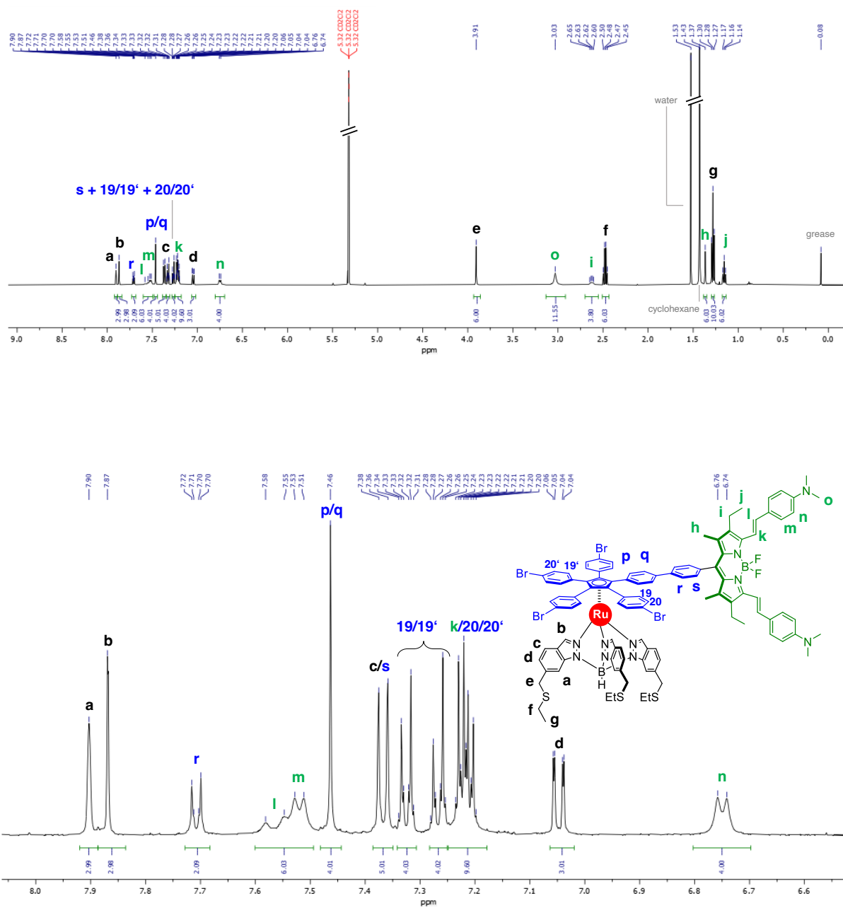
Fig. S9. 1 H NMR spectrum (500 MHz) of complex Br 4 B 2 [Ru] in CD 2 Cl 2 recorded at 25 °C and zoom of the 8.0-6.6 ppm region (bottom).
