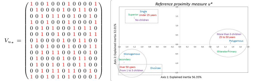
Fig. 3. TMCA - Adjacency matrix and Graphical representation
