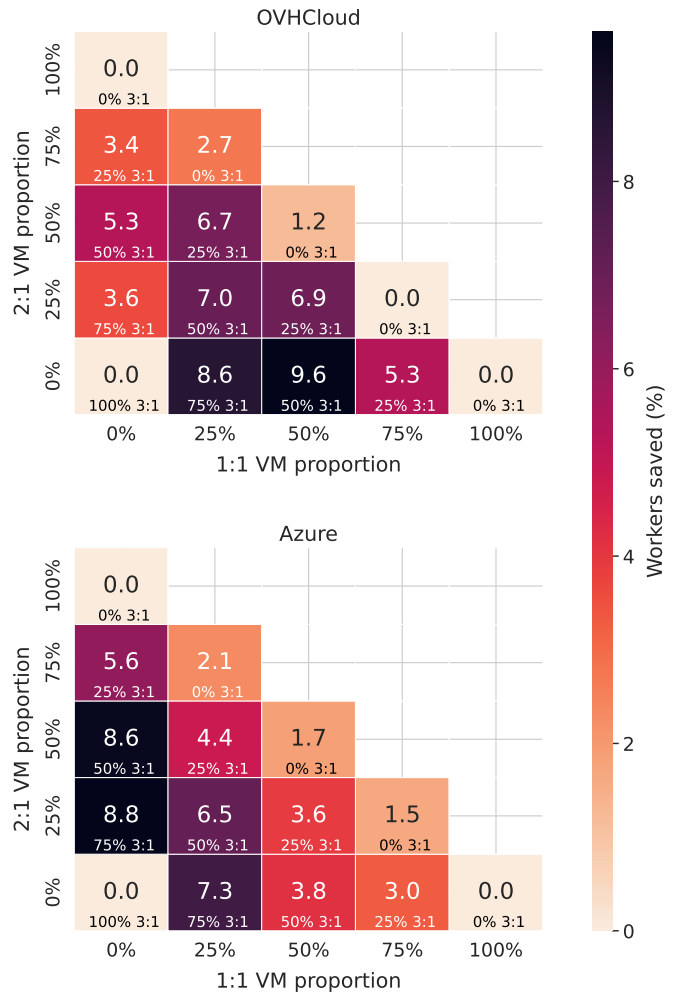
Fig. 4. SLACKVM gains in terms of PM (%) for various oversubscription distributions (the 3:1 VM distribution corresponds to the 100 complement of the other two distributions)
