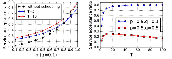
Fig. 11: Service acceptance ratio depending on T
