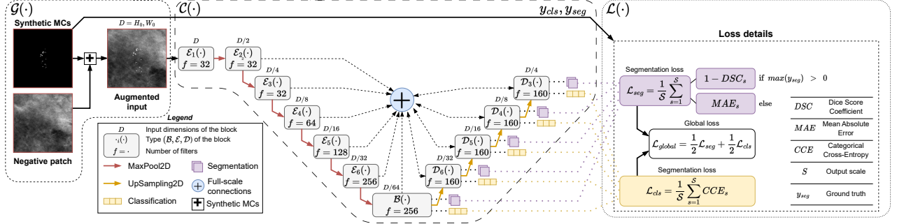
Figure 1. Overview of the proposed framework. Synthetic MCs are generated and inserted into a patch extracted from a negative exam and fed into the network. The CNN is based on multi-task and multi-scale approaches. Multi-classification and multi-channel segmentation tasks aim to distinguish soft tissues from benign and malignant MCs and are trained concurrently with \mathcal{L}_{global} loss. \mathcal{E}_n(\cdot) , \mathcal{B}(\cdot) , and \mathcal{D}_n(\cdot) denote the encoder, bottleneck and decoder at the n_{th} scale with f being number of filters.
