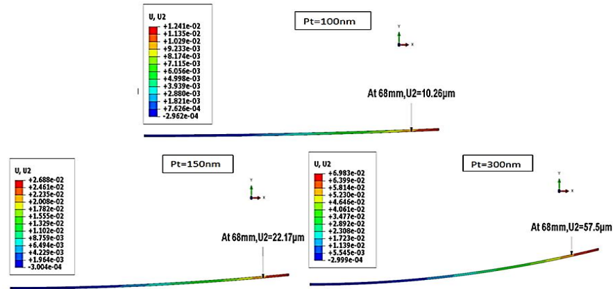
Figure 5. Warpage of the Si/USG/Pt stack using the full thermal cycle load.
