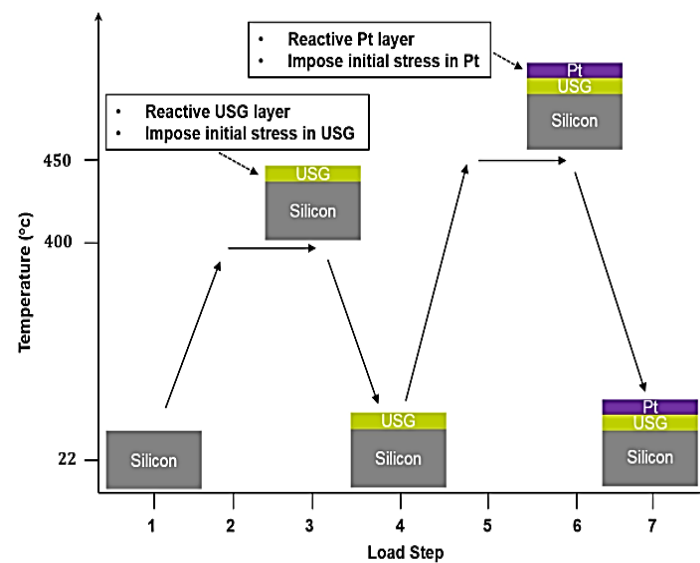
Figure 3. The whole thermal cycle used by Yao et al. [3].
