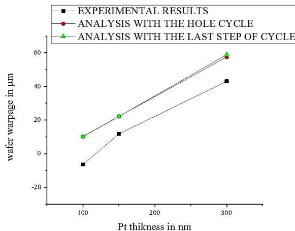
Figure 7. Numerical results and experimental measurements [3] of Si/USG/Pt warpage.
