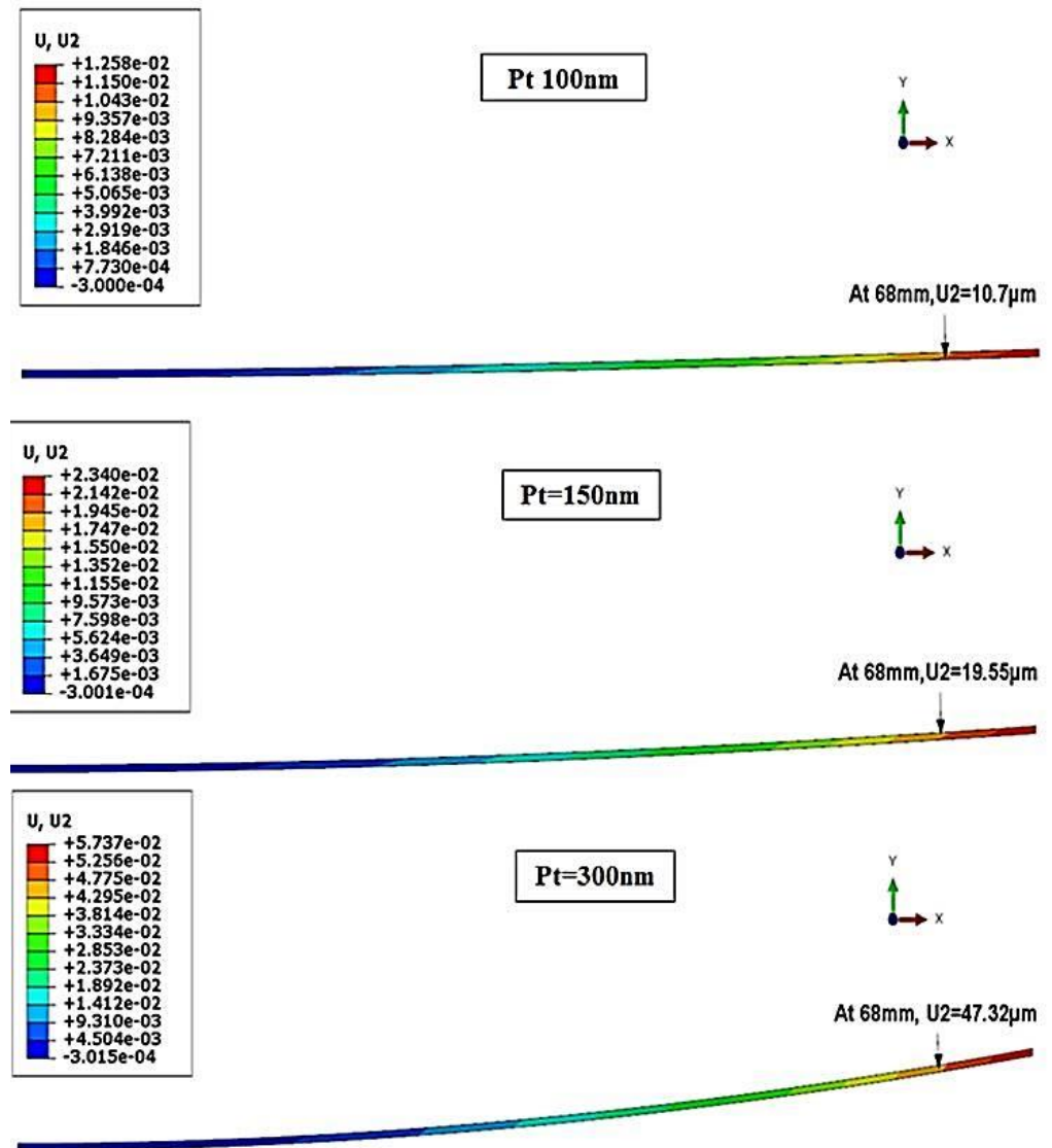
Figure 8. Warpage of the homogenized stack.
