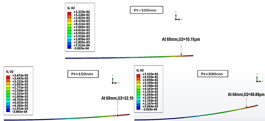
Figure 6. Warpage of the Si/USG/Pt stack using the last step of the full thermal cycle.
