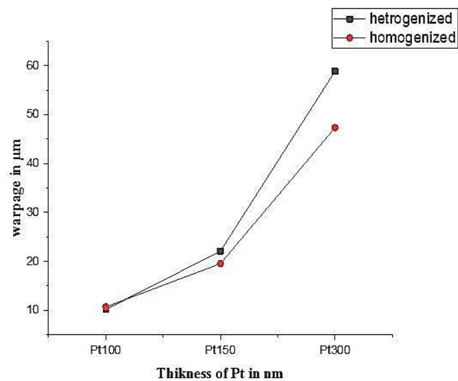
Figure 9. Warpage obtained using the homogenized/heterogeneous model.
