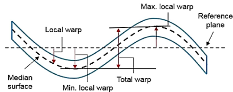
Figure 1. Illustration of the warping measurement method [3].
