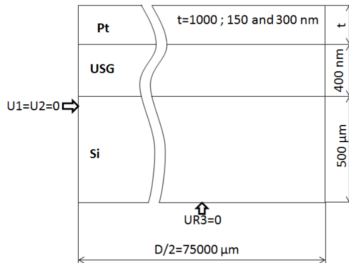
Figure 2. Geometry and boundary conditions of the 2D axisymmetric model.
