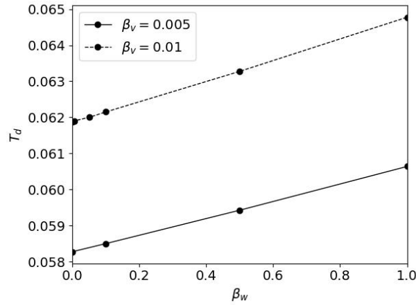
Figure 7: T_d as a function of \beta_w for \Xi = 5 and \beta_v = 0.005, 0.01 .
