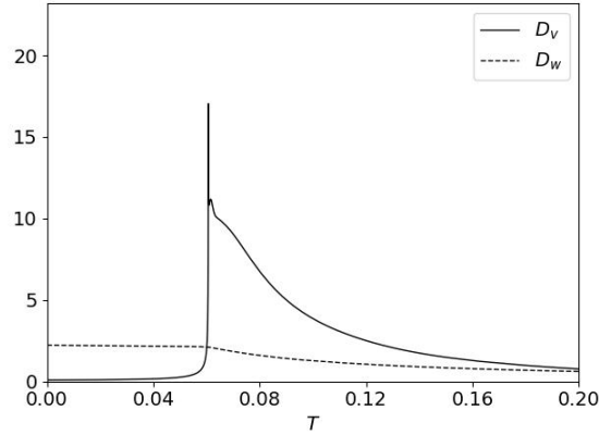
Figure 3: Evolution of D_w and D_v for \Xi = 5 , \beta_w = 2 and \beta_v = 0.002 .
