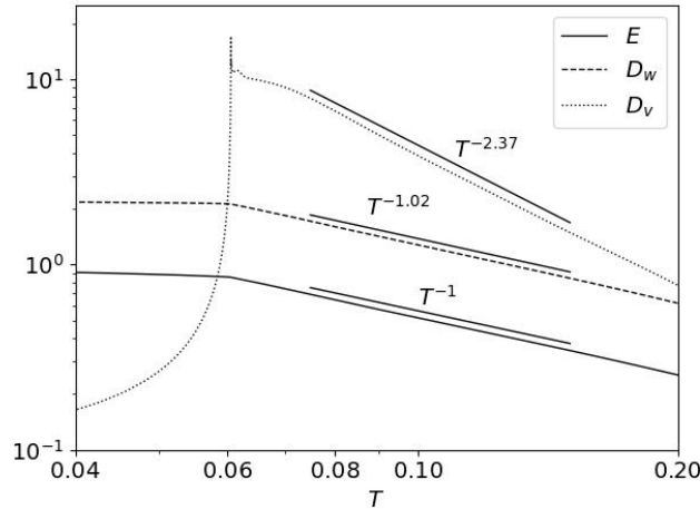
Figure 8: Log-log plots of E , D_w and D_v as a function of T for \Xi = 5 , \beta_w = 2 and \beta_v = 0.002 .
