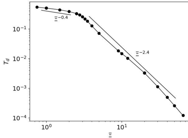
Figure 9: Log-log plot of T_d as a function of \Xi for \beta_w = 1 and \beta_v = 0.01 .
