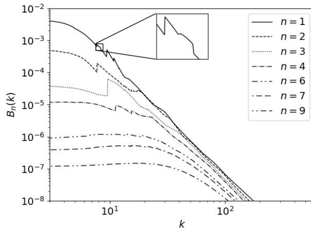
Figure 13: Log-log plots of B_n(k) as a function of k for \Xi = 5 , \beta_w = 1 , \beta_v = 0.01 , different values of n and T = T_d = 0.0648 .
