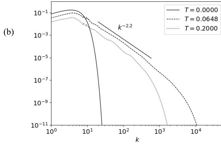
Figure 14: Log-log plots of (a) e_n as a function of n and (b) e(k) as a function of k for \Xi = 5 , \beta_w = 1 and \beta_v = 0.01 at different times.
