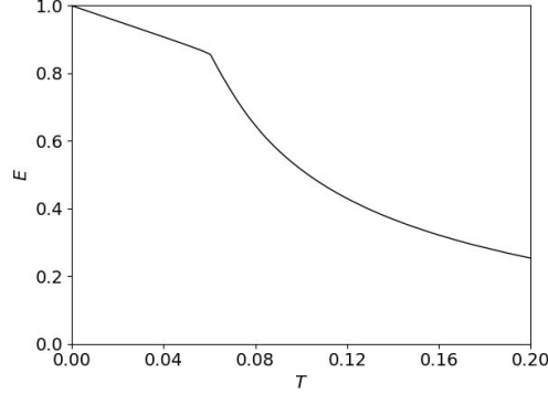
Figure 2: Evolution of the wave energy for \Xi = 5 , \beta_w = 2 and \beta_v = 0.002 .
