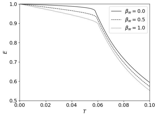
Figure 6: Evolution of the wave energy for \Xi = 5 , \beta_v = 0.005 and different values of \beta_w .
