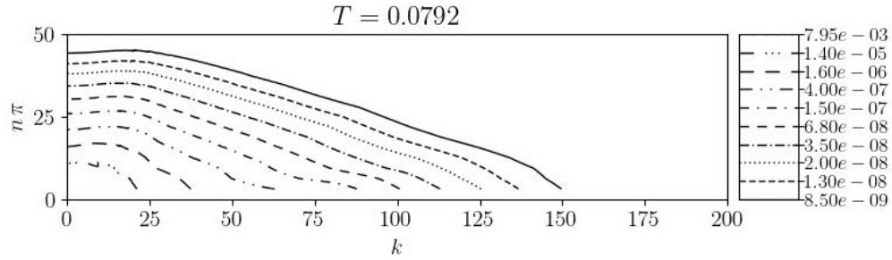
Figure 12: Contour plots of B_n(k) in the k - n\pi plane for \Xi = 5 , \beta_w = 1 , \beta_v = 0.01 and different values of T , the first of which is at the initial time, the second just prior to T = T_d , the third at T = T_d and the fourth at a significantly greater time. Of course, the plots only show data for integers n \geq 1 . Thus, they only extend down to \pi on the vertical axis.
