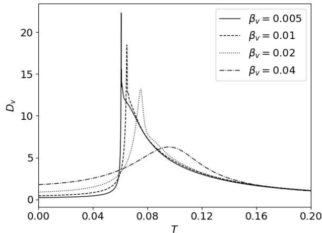
Figure 5: Evolution of D_v for \Xi = 5 , \beta_w = 1 and different values of \beta_v .
