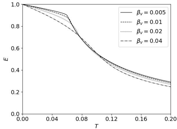
Figure 4: Evolution of the wave energy for \Xi = 5 , \beta_w = 1 and different values of \beta_v .
