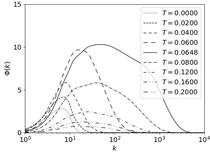
Figure 16: The spectral flux, \Phi(k) , as a function of k for \Xi=5 , \beta_w=1 and \beta_v=0.01 at different times. The horizontal axis is logarithmic, while the vertical one is linear.
