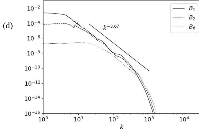
Figure 10: Log-log plots of B_1(k) , B_2(k) and B_6(k) for \Xi = 5 , \beta_w = 2 and \beta_v = 0.005 at times (a) T = 0 , (b) T = 0.031 , (c) T = 0.0633 and (d) T = 0.2 . The spectral front advances in (a), (b), (c) and retreats in (c), (d). The straight lines in (c) and (d) represent the power law k^{-3.67} .
