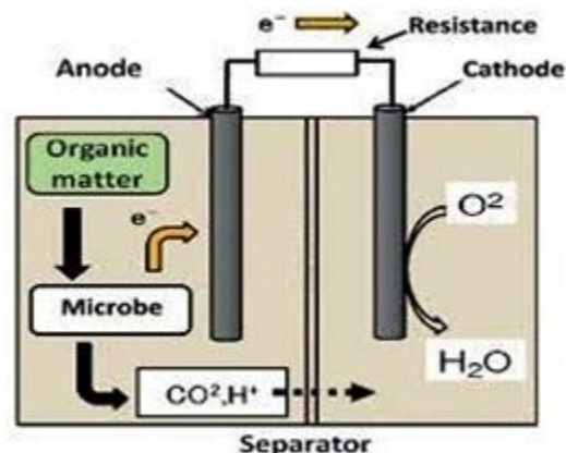
Fig. 5 Schematic representation of microbial fuel cell
