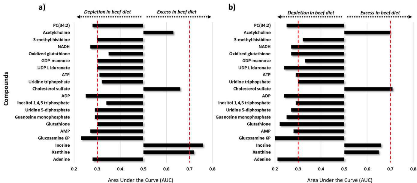
Fig. 3. Area Under the Curve (AUC) values of discriminant metabolites between red and white meat diets for (a) the epithelium part and for (b) the top of the crypts.
