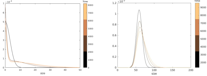
(a) Size distribution c(j, t) when v = w > \epsilon , i.e. for t = 0, T_0, T_1, T_2 . (b) Size distribution c(j, t) when v = w < \epsilon , i.e. for t \approx \Delta t, T_0 + \Delta t, T_1 + \Delta t, T_2 + \Delta t .
