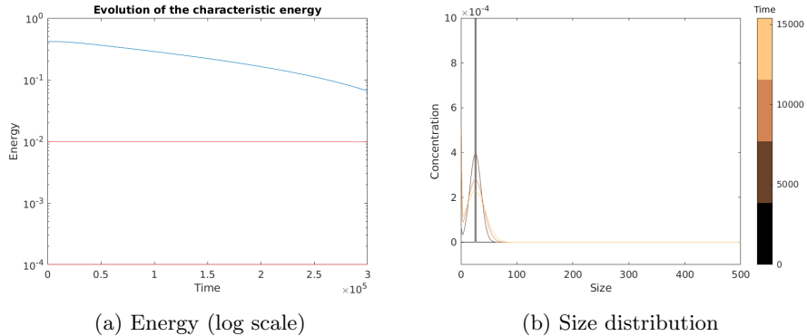
Figure 10: Numerical simulation of the evolution of the cluster size distribution and the energy taking as initial condition a Dirac mass located at the size R_\varepsilon = 25 and v = w \approx \frac{1-a}{2} . The time evolution is indicated by the colors in Figure 10b. The Figure 10b is truncated on the y-axis at 0.001. In the Figure 10a, the horizontal red lines illustrate the thresholds when the energy would be inferior to \varepsilon .
