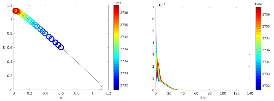
(c) Phase portrait of (v, w) for t \in [T, T + t_1] = [2733, 2736] , cf. Lemma 2.2 (d) Evolution of cluster distribution c(j, t) for t \in [T, T + t_1] = [2733, 2736]
