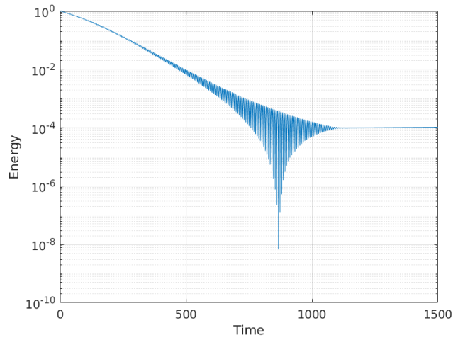
Figure 9: Numerical simulation of the time evolution of the Energy \tilde{E} defined in (81) during Phase III and the beginning of Phase IV. The time t = 0 corresponds to the end of Phase II and the beginning of Phase III in this simulation. The y-axis is logarithmic and \varepsilon = 0.02 . The decay of the energy is exponential-like until it reaches an order of magnitude of \varepsilon^2 \approx 10^{-4} ; the order of magnitude of the energy oscillations then become of the same order of magnitude as the energy itself, and then decay (end of Phase III).
