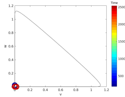
(c) Phase portrait of (v, w) for t \in [t_2, t_3] = [191, 2541] , cf. Lemma 2.4
