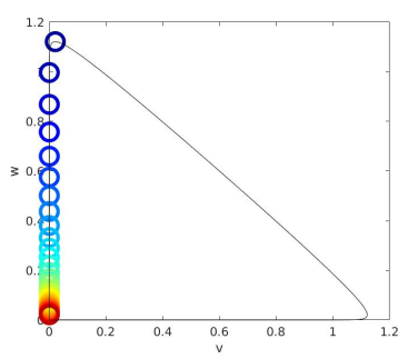
(a) Phase portrait of (v, w) for t \in [t_1, t_2] = [3, 191] , cf. Lemma 2.3
