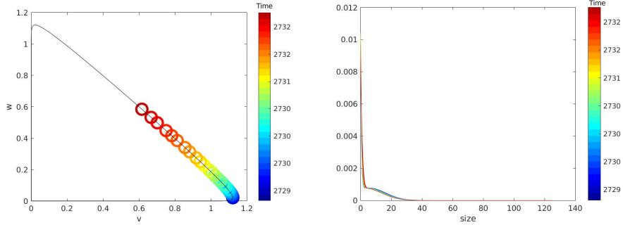
(a) Phase portrait of (v, w) for t \in [t_4, t_5 = T] = [2729, 2732] , cf. Lemma 2.6 (b) Evolution of cluster distribution c(j, t) for t \in [t_4, t_5 = T] = [2729, 2732]
