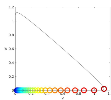
(e) Phase portrait of (v, w) for t \in [t_3, t_4] = [2541, 2729] , cf. Lemma 2.5
