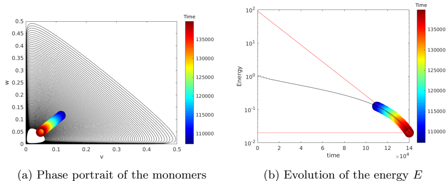
Figure 7: Numerical simulation of the evolution of the monomers and the energy in Phase II (c.f section 4.1). The color scheme indicates the time evolution in Figures 7a and 7b. (Right) The y-axis scale is logarithmic and the horizontal line is E_n \approx \varepsilon where \varepsilon = 0.02 in the numerical simulation. The decreasing affine line in red is an illustration of the exponential decay of the energy that takes place in Phase II (see Prop. 4.3).
