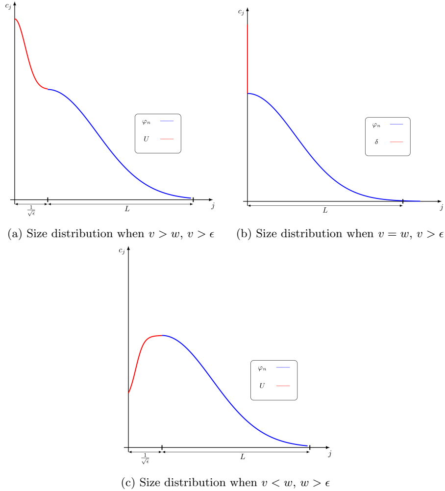
Figure 4: Scheme of the evolution of the cluster sizes of order one.
