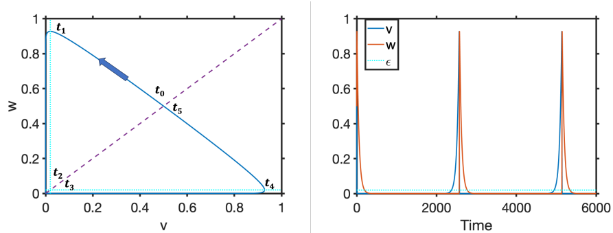
Figure 1: Numerical solution of the Lotka-Volterra system (14) for \varepsilon = 0.02 and v(0) = w(0) = \frac{1}{2} . To avoid numerical dissipation we rather solved the system for (\log(v), \log(w)) , see Appendix C.1, System (144). Left: phase portrait for (v, w) illustrating the different stages of the trajectory over one period T . The dashed purple line is the subset where v = w , the dotted blue lines are w = \varepsilon or v = \varepsilon . Right: time-evolution of the solution (v, w) .
