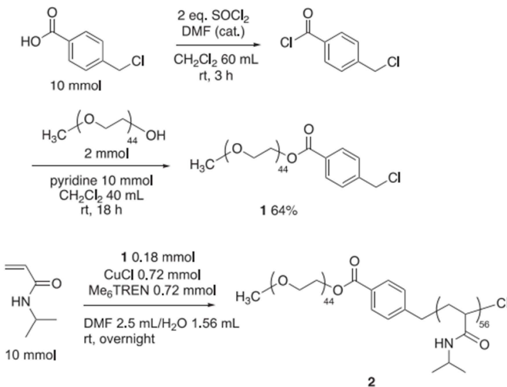
Scheme 1. Preparation of NIPAAm- b -PEG 2 with PEGylated ATRP agent. Reprinted with permission of Elsevier from [70]. Copyright 2019.
