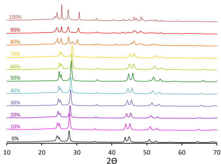
Figure 1: X-ray diffraction pattern of Tb doped LaF 3 NPs. The percentages indicated correspond to the Tb doping rates in the NPs.
