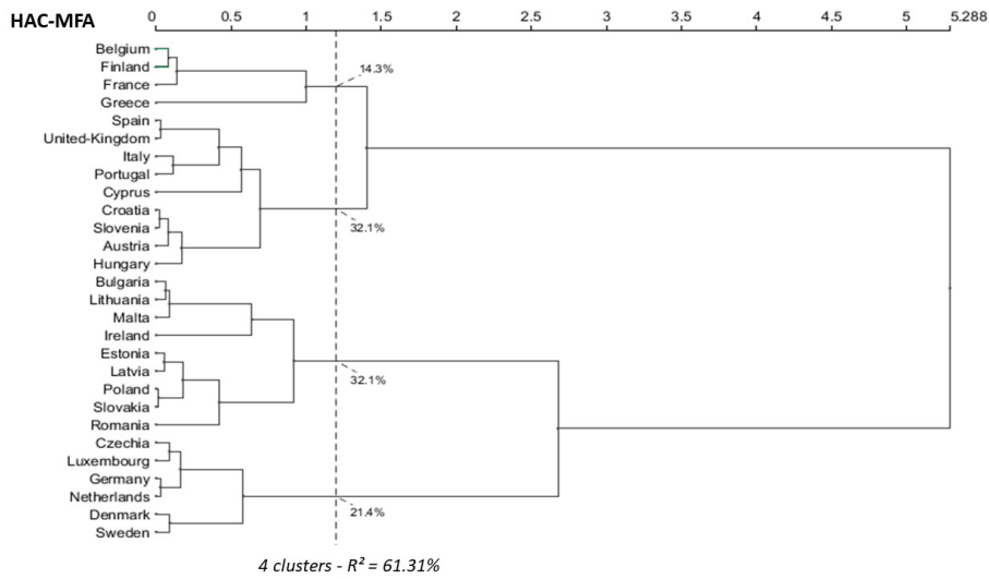
Fig. 4. Topological and HAC-MFA cluster dendrograms of the EU-28 countries
