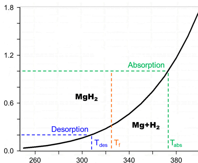
Figure 11. Equilibrium diagram of the system \text{Mg} + \text{H}_2 \leftrightarrow \text{MgH}_2 showing a melting temperature T_f of the PCM intermediate between the absorption ( T_{abs} ) and desorption ( T_{des} ) temperatures of the compacts.
