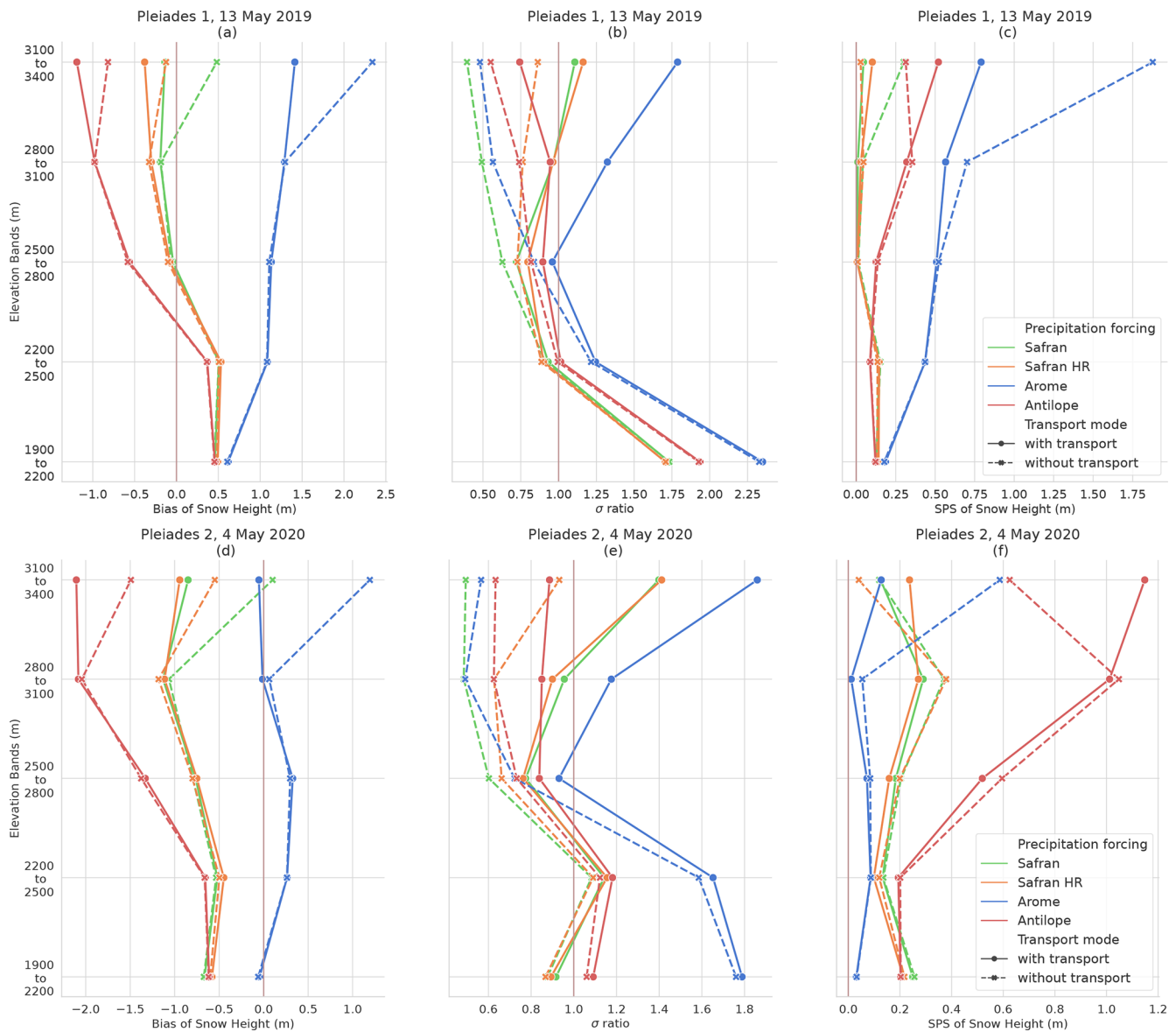
Figure 6. Scores comparing simulations with the Grandes Rousses Pléïades observations. Panels (a), (b), and (c) compare simulations with the 13 May 2019 Pléïades 1 image; panels (d), (e), and (f) are based on the 4 May 2020 Pléïades 2 image. (a), (d) Bias (m); (b), (e) standard deviation ratio (no unit); (c), (f) SPS (m). All scores are presented as a function of 300 m elevation intervals.
