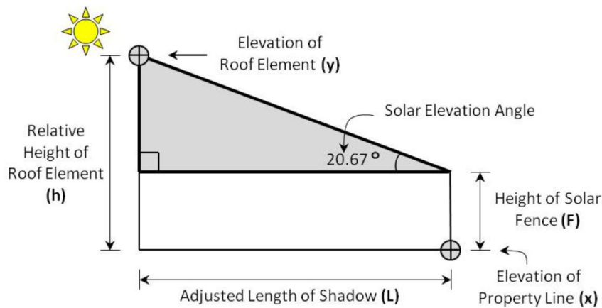
Figure 17: Section along Shadow Length at 10 AM
