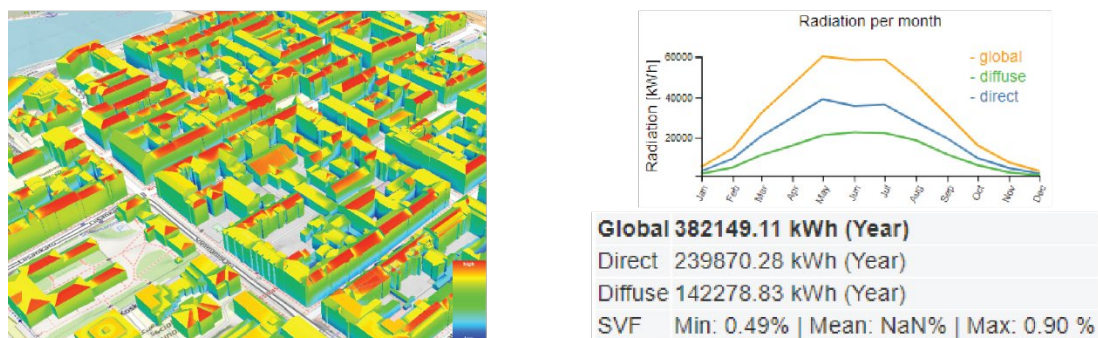
Figure 9: Solar Energy Potential map of Helsinki
