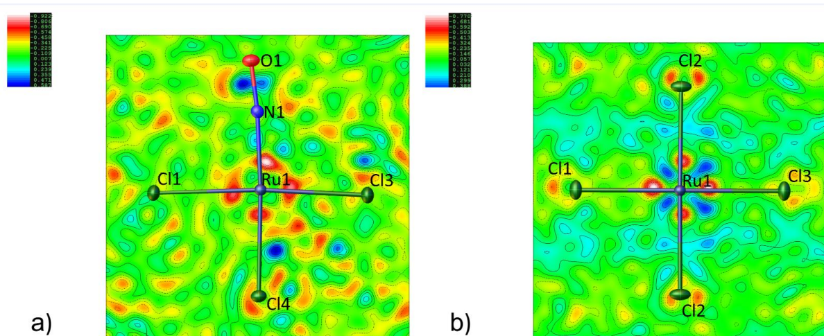
Fig. S1. Fourier-difference maps for K_2[RuCl_5NO] . a) Plane containing the RuNO axis, illustrating the depletion of the Ru 4d_{z^2} orbital. b) Equatorial plane, illustrating the depletion of the Ru 4d_{x^2-y^2} and population of the Ru 4d_{xy} .
