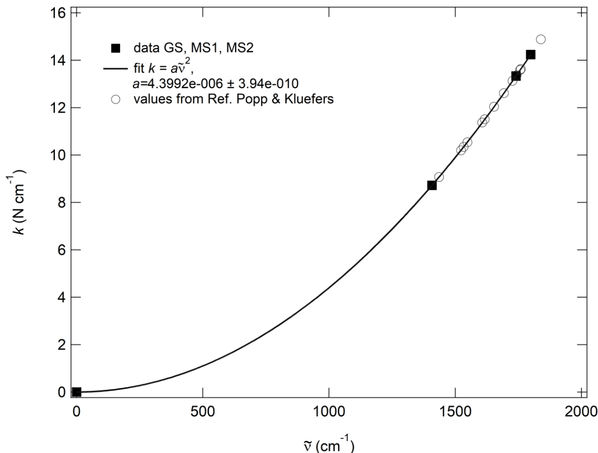
Fig. 7. Quadratic dependence k^{dc} = a(\tilde{\nu}^{dc})^2 , ( a=4\pi^2c^2\mu ) for the NO stretching vibration of GS, MS1, and MS2 in K_2[RuCl_5NO] , resulting from the decoupling into two-atomic harmonic oscillators. For the fit, the point k = \tilde{\nu} = 0 has been added.
