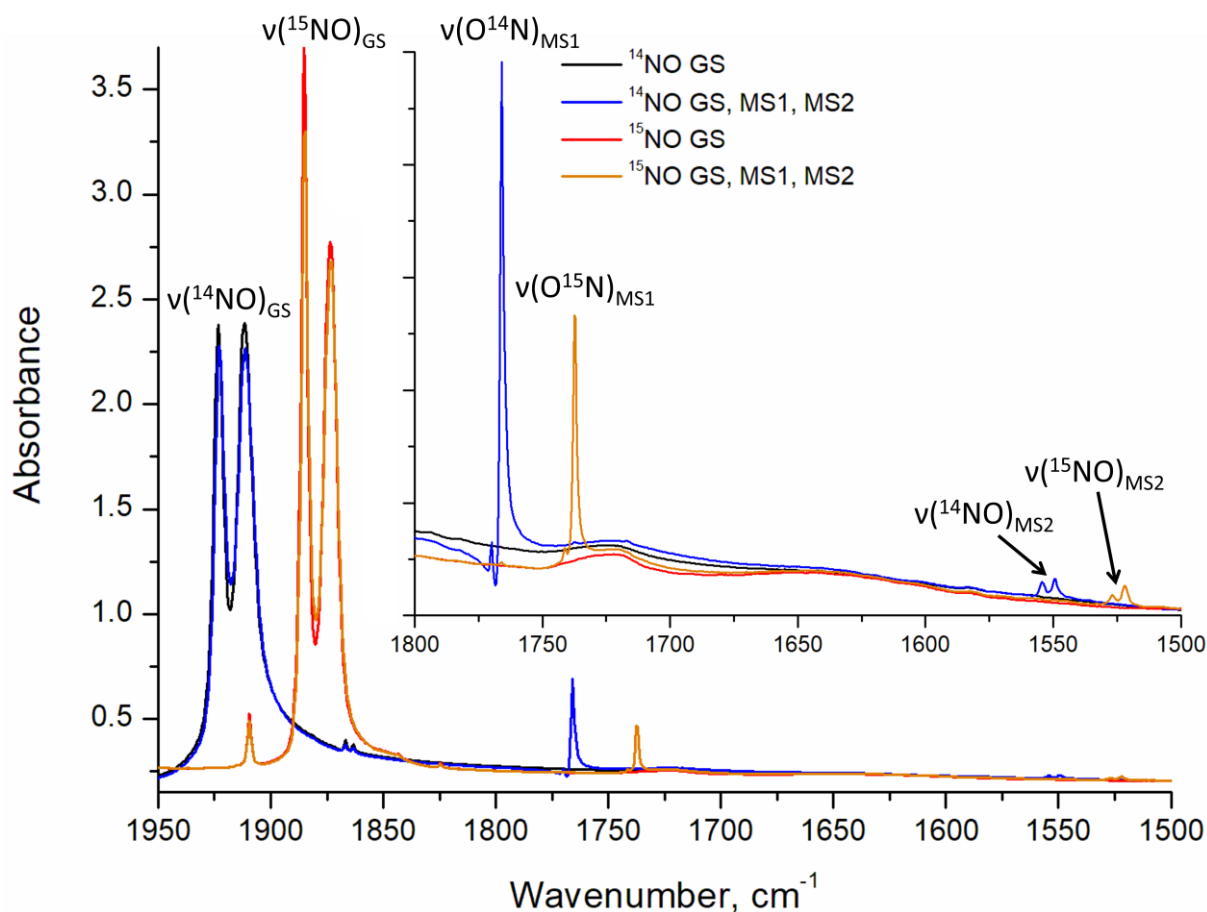
Fig. 5: Comparison of the experimentally observed vibrations of GS, MS1 and MS2 in the spectral range of 1950–1500 \text{cm}^{-1} . The spectra were measured at 10 K, MS1 and MS2 were photogenerated by irradiation at 520 nm.
