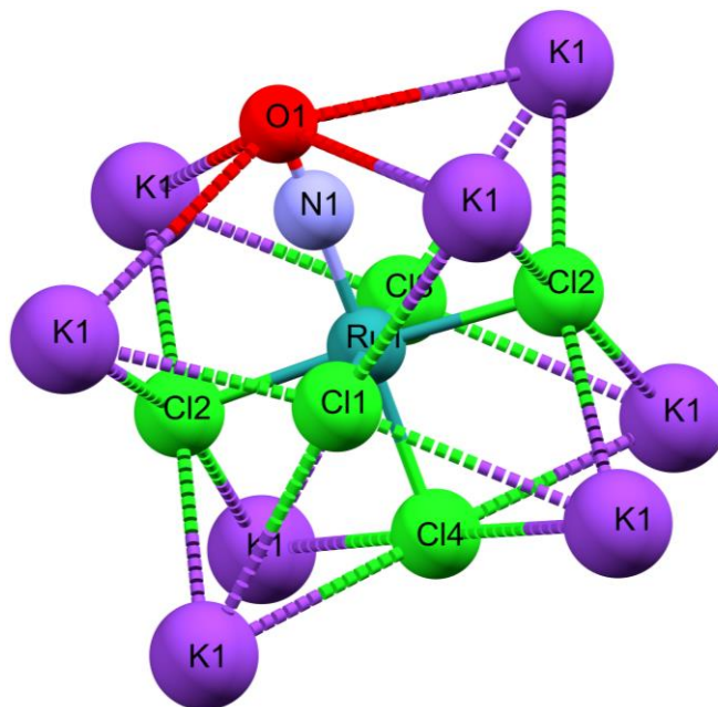
Fig. 2: Cationic K^+ environment for the [RuCl_5NO]^{2-} anion.
