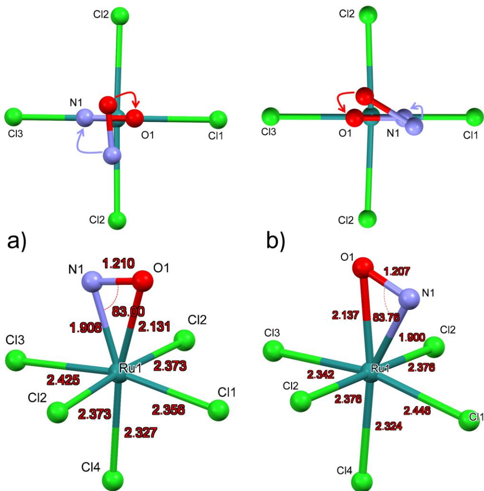
Fig. 4: Calculated structural model of [\text{RuCl}_5\text{NO}]^{2-} in MS2: a) Initial and converged structure of MS2 converging O atom of NO towards Cl1 ligand; b) initial and converged structure of MS2 converging O atom of NO towards Cl3 ligand.
