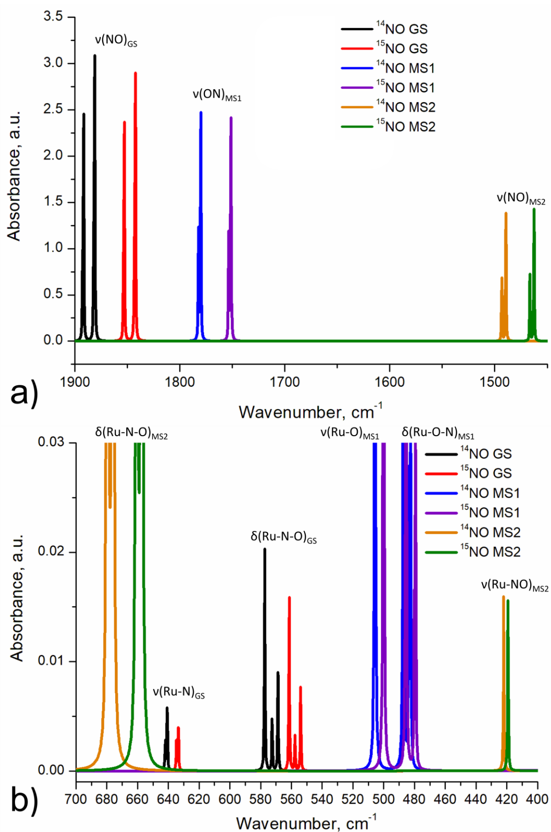
Fig. S5. CASTEP-calculated IR spectra of GS, MS1 and MS2 in spectral ranges of 1900–1450 (panel a) and 700–400 \text{cm}^{-1} (panel b).
