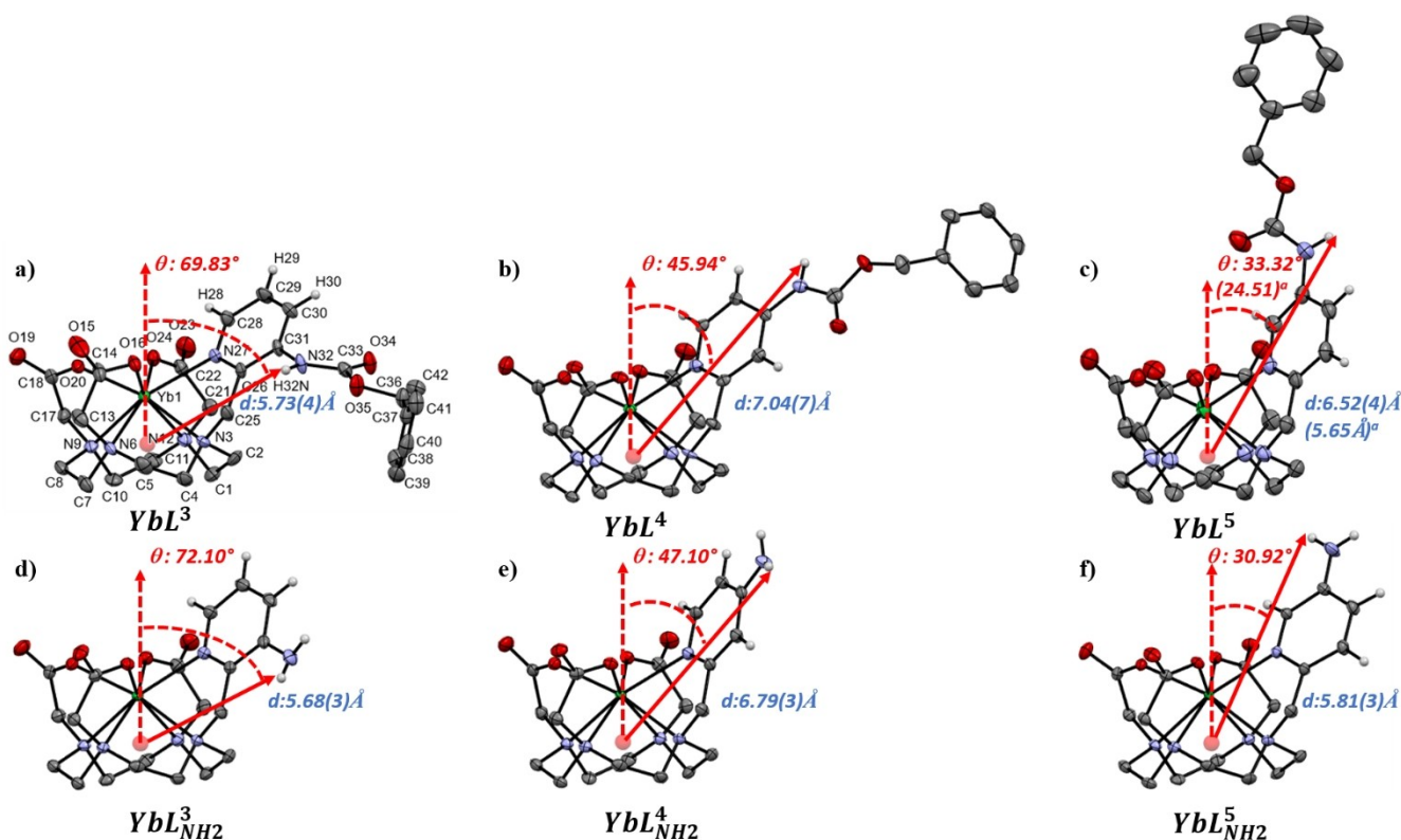
Figure 1. ORTEP-III plots [42] of enantiomers \Delta(\delta\delta\delta\delta) in the unit cell of the complexes a) YbL^3 , b) YbL^4 , c) YbL^5 , d) YbL^3_{NH_2} , e) YbL^4_{NH_2} and f) YbL^5_{NH_2} (generated from CIF files using the Mercury software [43] ). Ellipsoids are drawn at the 50% probability level and, for clarity, H atoms of the macrocycle and solvent molecules are not shown. The side-on views of all the complexes are given with the same orientation. Dashed red arrow: axis passing through the N 4 macrocycle centroid (orange sphere) and Yb 3+ , solid red arrow: vector linking N 4 macrocycle centroid to the carbamate or amine protons; \theta : angle between these two axes; d : distance from the Yb 3+ to the amine or carbamate proton. [a] calculated for the assumed solution structure of YbL^5 .
