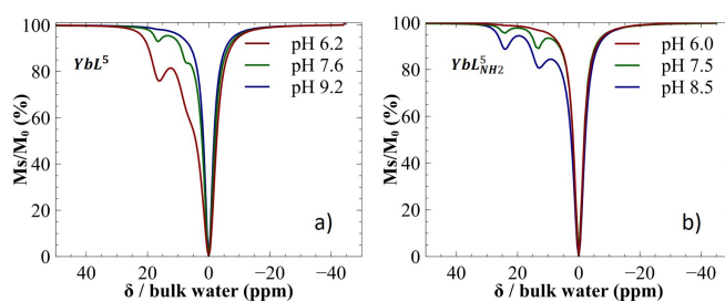
Figure 3. pH-dependent CEST spectra of 15.9 mM and 18.3 mM solutions of \text{YbL}^5 (a) and \text{YbL}_{\text{NH}_2}^5 (b), respectively (400 MHz, 25 \mu\text{T} saturation power during 3 s, \text{H}_2\text{O}/\text{D}_2\text{O} ).
