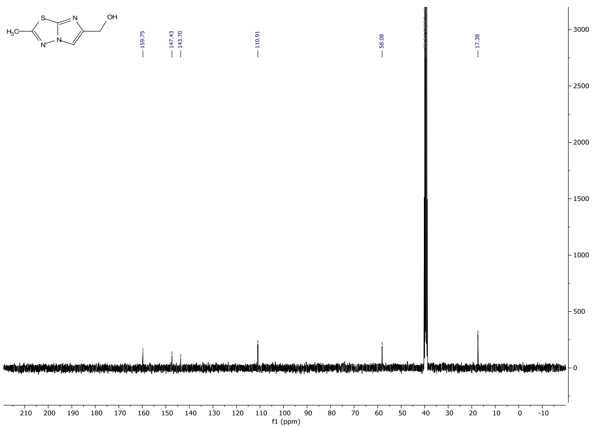
Figure S1 : ^1\text{H} and ^{13}\text{C} NMR spectra of compound 3 .
